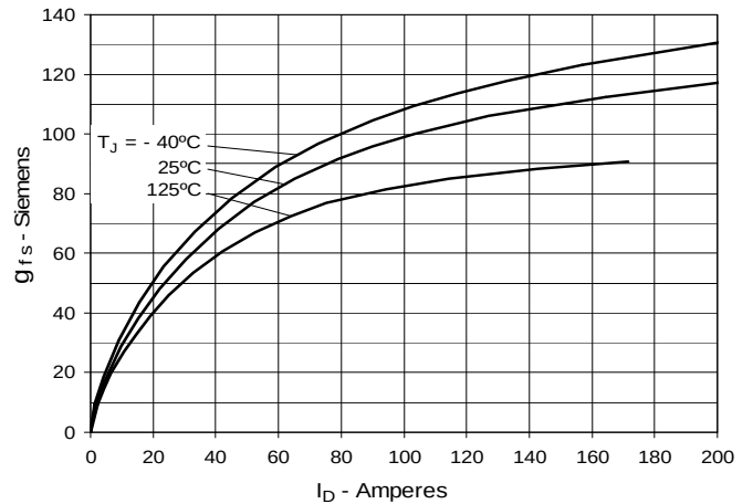
Fig. 8. Transconductance
