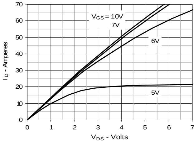
Fig. 1. Output Characteristics @ 25°C
