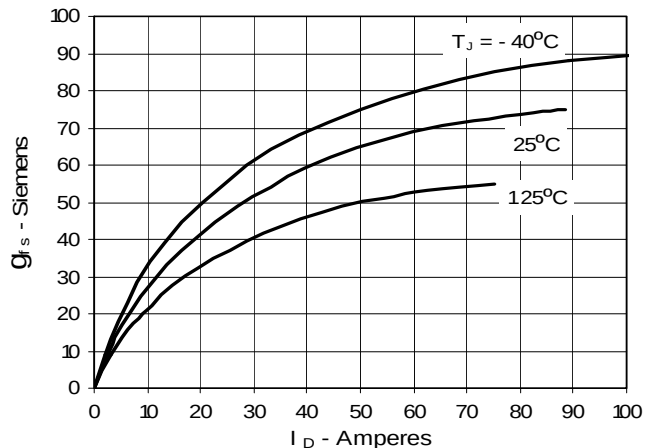
Fig. 8. Transconductance
