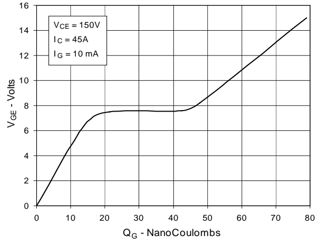
Fig. 14. Gate Charge
