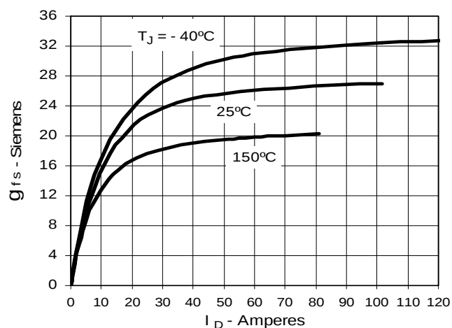
Fig. 8. Transconductance
