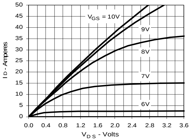
Fig. 3. Output Characteristics
