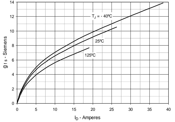
Fig. 8. Transconductance
