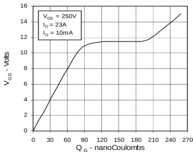
Fig. 10. Gate Charge
