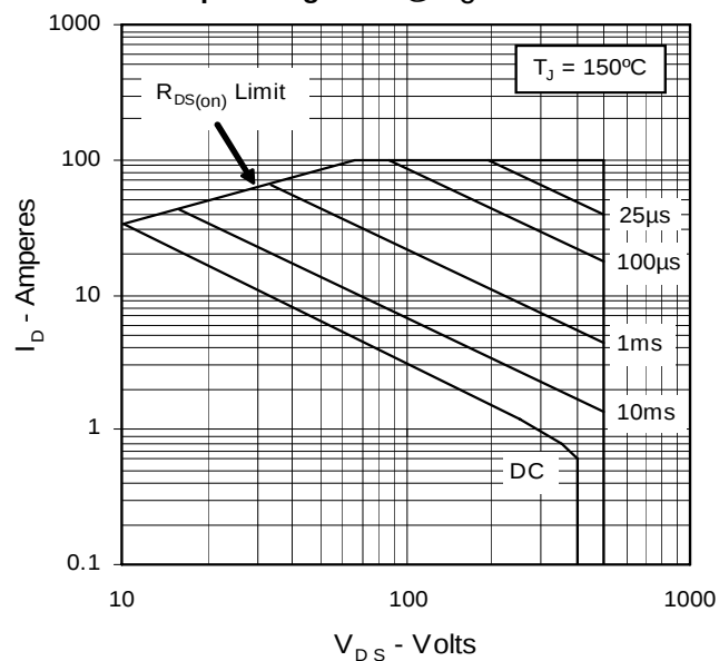
Fig. 13. Forward-Bias Safe Operating Area @ T_C = 90^\circ\text{C}
