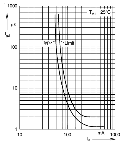
Fig. 1 Gate trigger delay time
