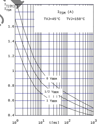
Fig. 2 Surge overload current per diode or thyristor I_{FSM}, I_{TSM} : Crest value t: duration
