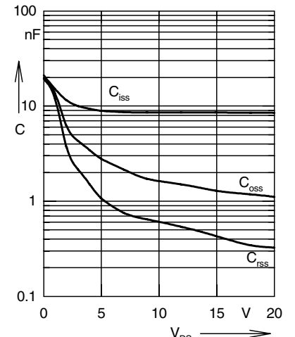
Fig. 6 Typ. capacitances C = f(V_{DS}) , f = 1 MHz (MOSFET)
