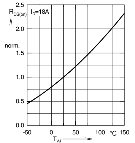
Fig. 3 Typ. normalized R_{DS(on)} = f(T_{VJ}) (MOSFET)
