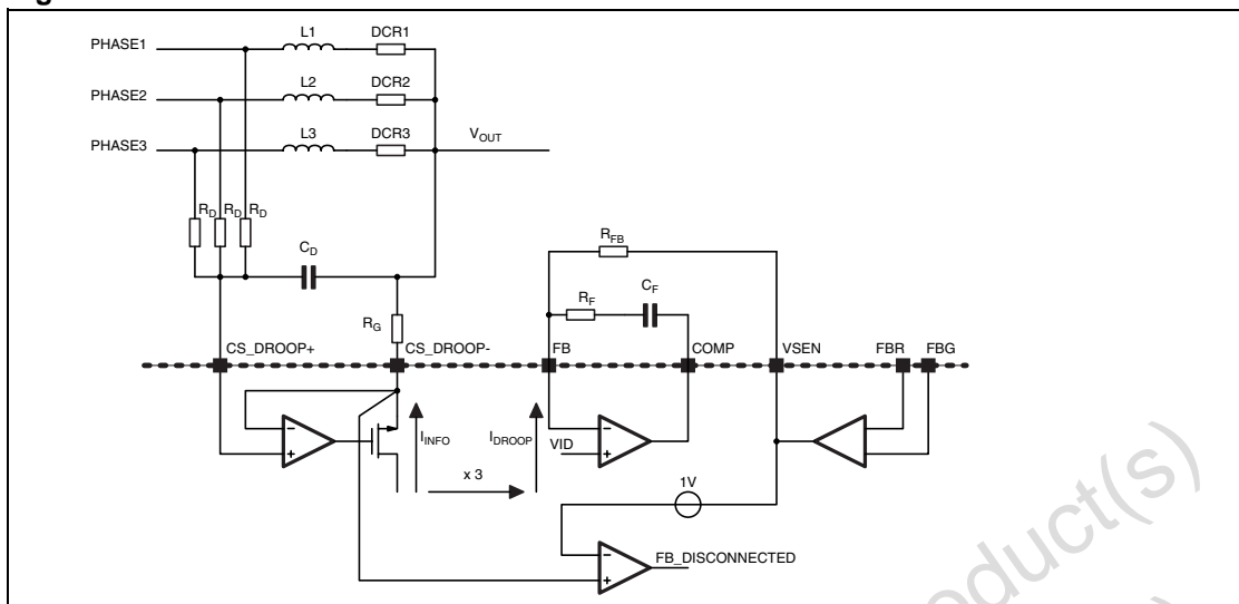
Figure 14. Feedback Disconnection
