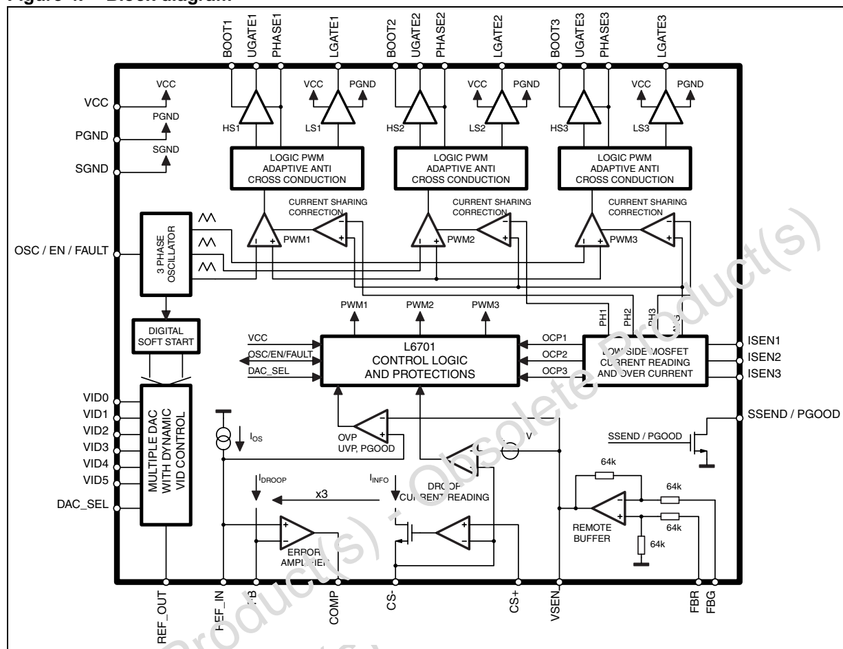
Figure 4. Block diagram
