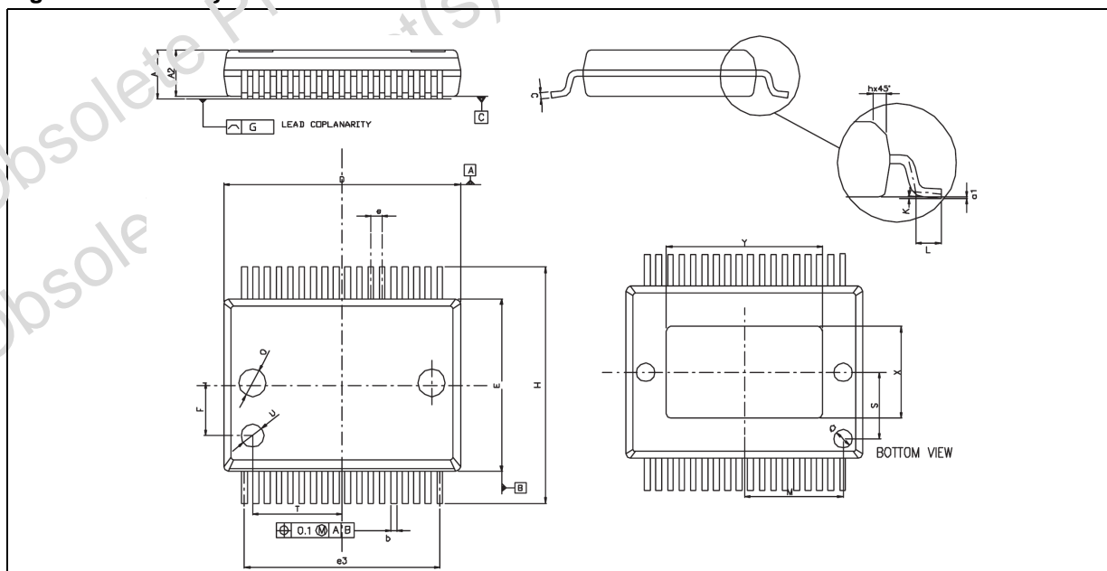
Figure 21. Package Dimensions
