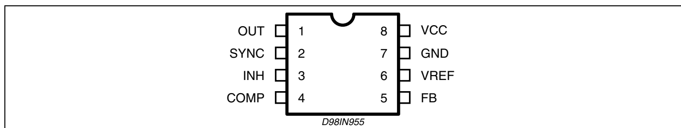
Figure 3. Pin Connection (top view)
