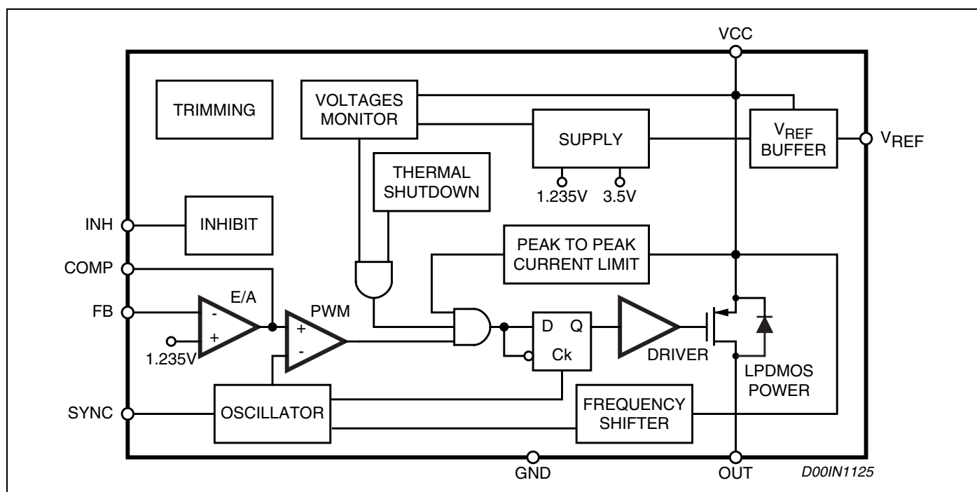
Figure 4. Block Diagram
