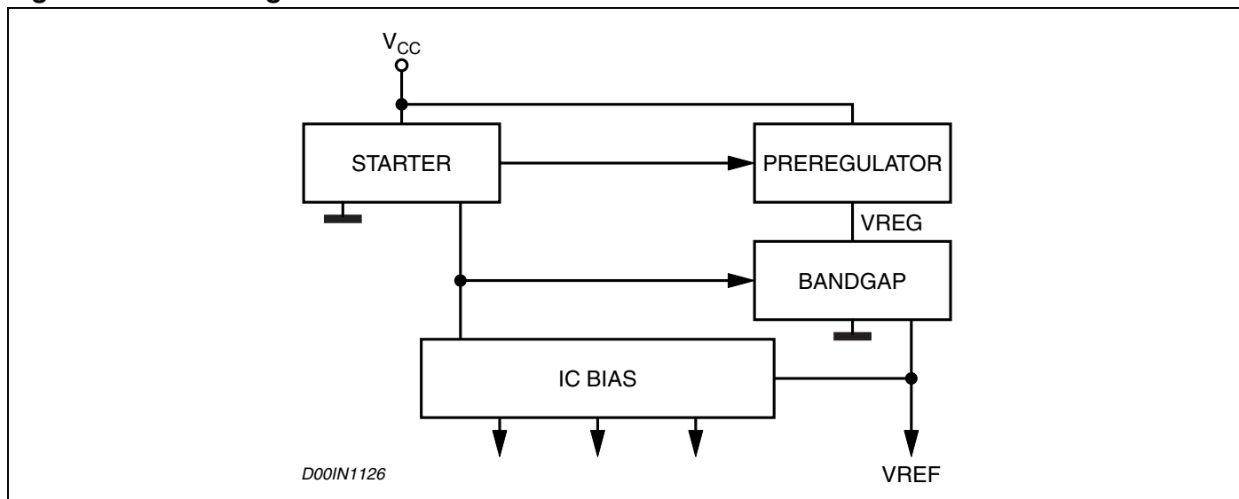
Figure 5. Internal Regulator Circuit
