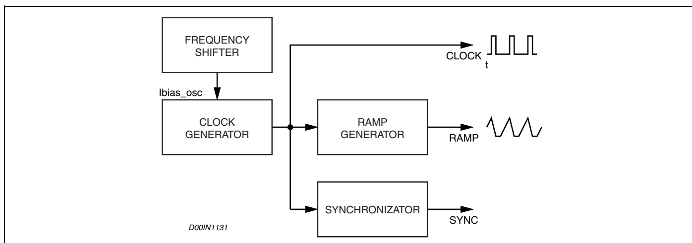
Figure 6. Oscillator Circuit
