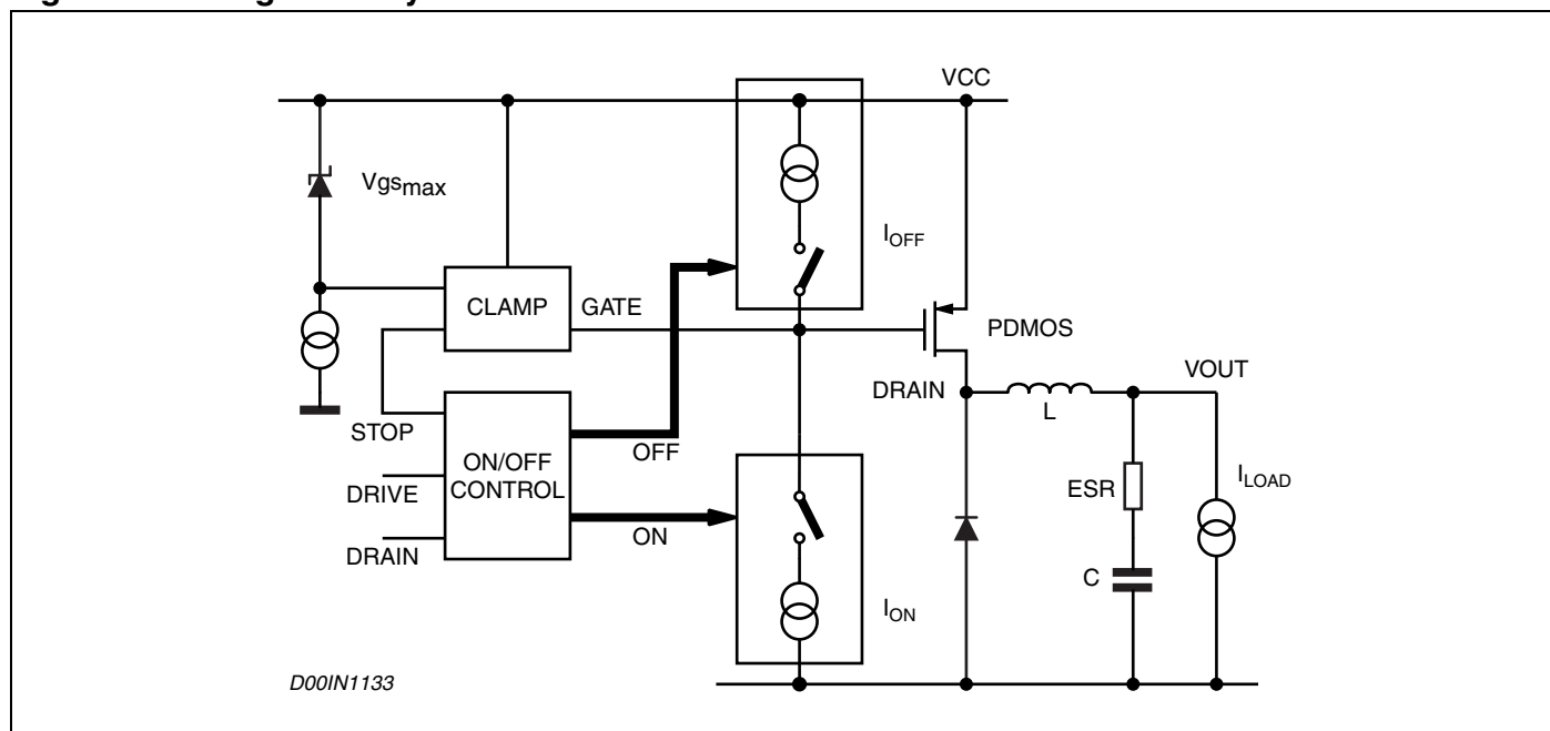
Figure 8. Driving Circuitry
