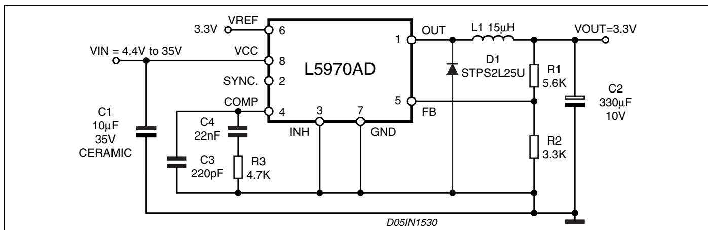
Figure 2. Test and Application Circuit
