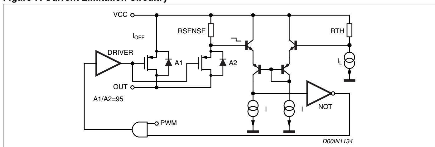
Figure 7. Current Limitation Circuitry
