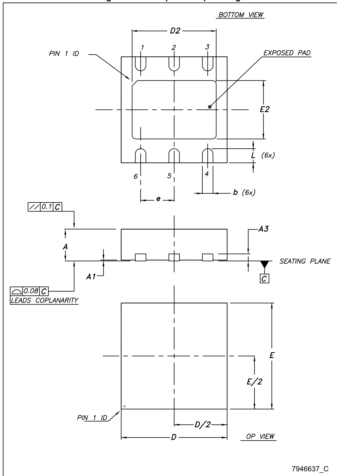
Figure 22. DFN6 (3 x 3 mm) drawings
