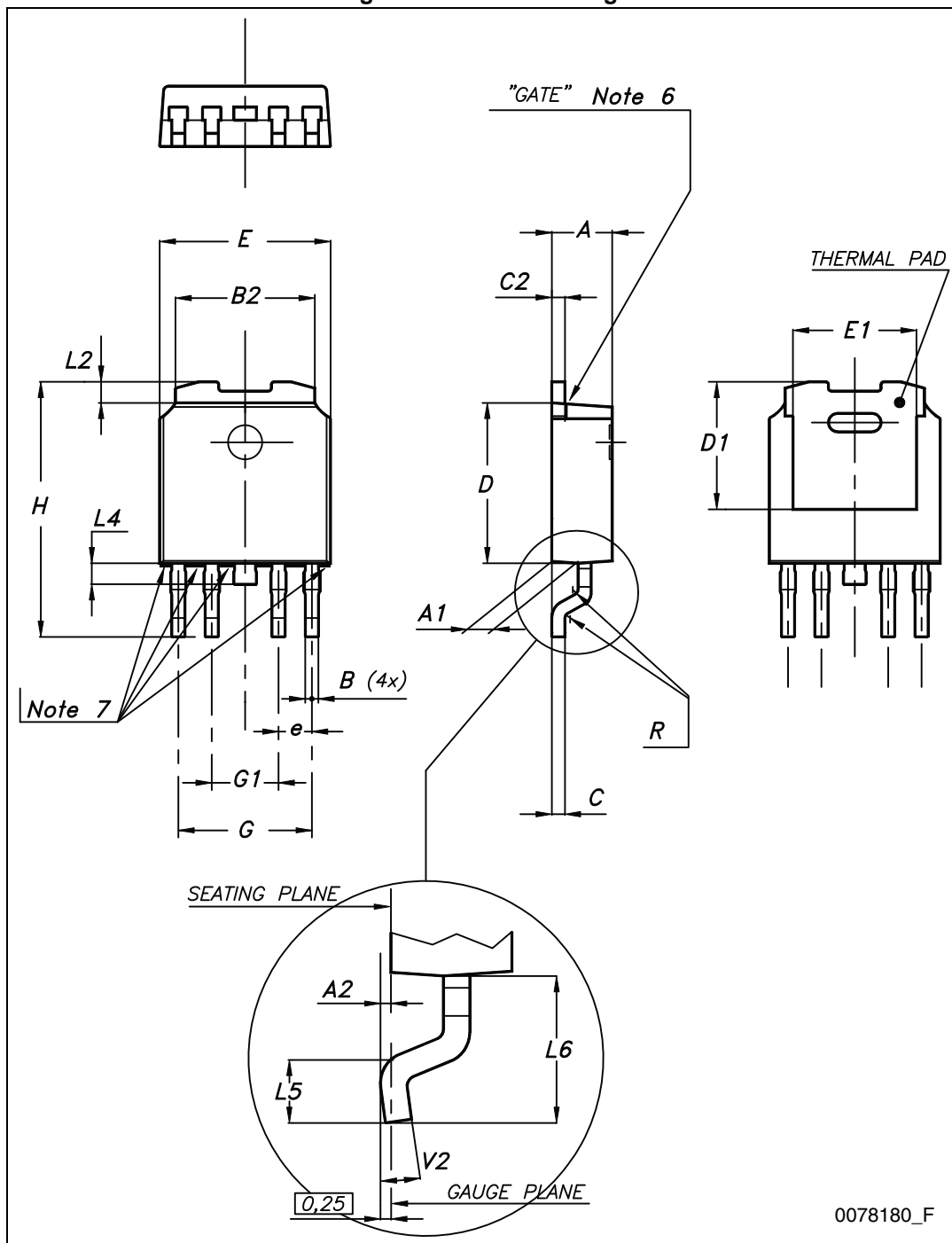
Figure 19. PPAK drawings
