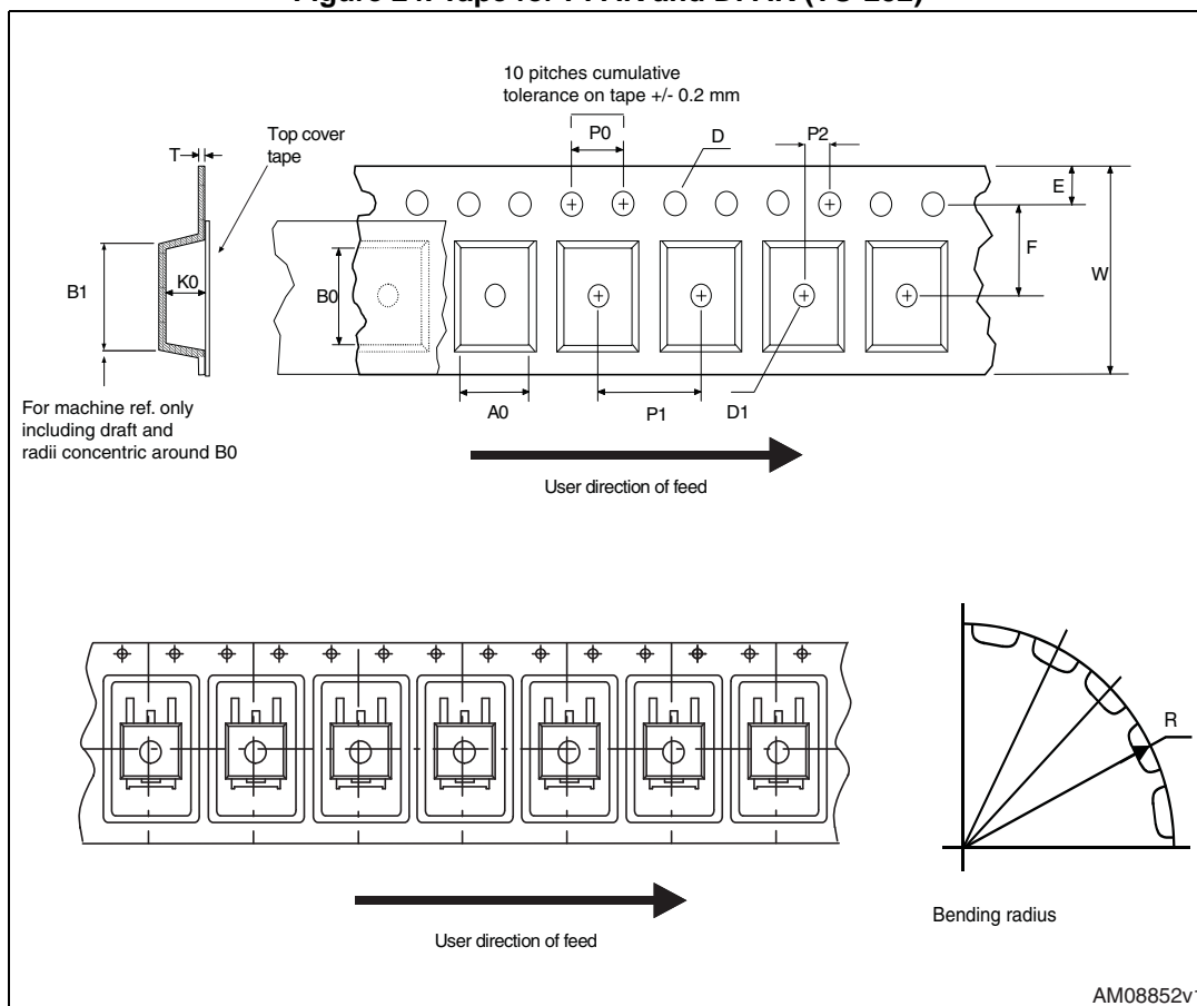
Figure 24. Tape for PPAK and DPAK (TO-252)
