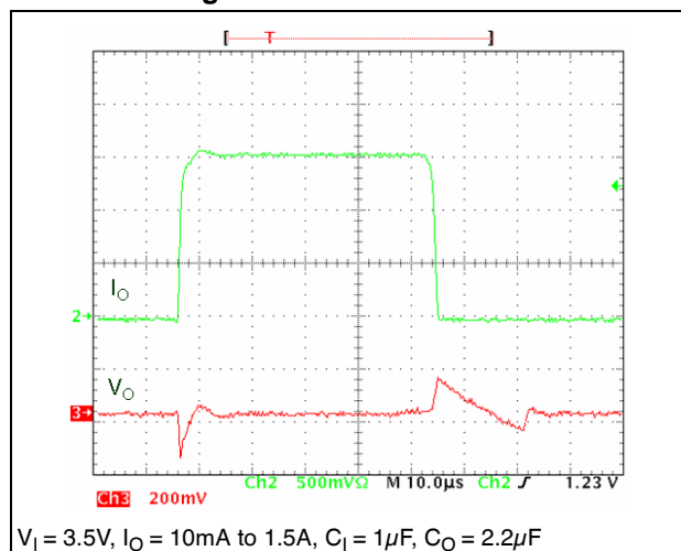
Figure 17. Load transient
