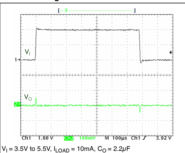
Figure 18. Line transient
