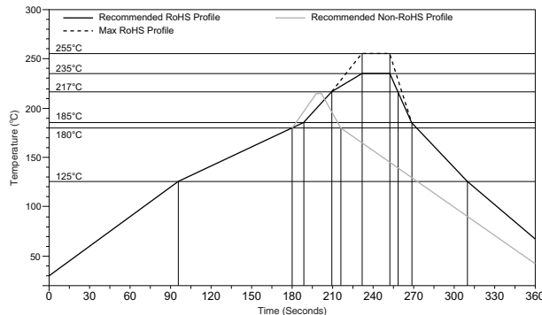
Figure 31: Maximum Reflow Temperature Profile
