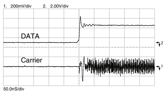
Figure 13: TX Modulation Delay
