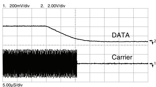
Figure 16: TX Turn-Off Time
