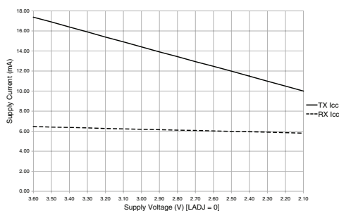
Figure 8: Current Consumption vs. Supply
