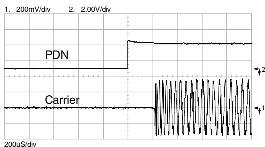
Figure 14: TX Turn-On Time from PDN
