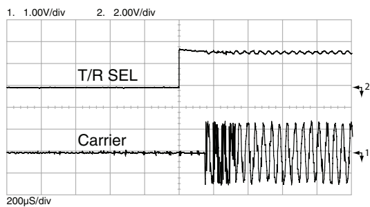
Figure 9: RX to TX Change Time
