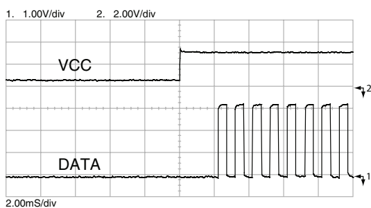
Figure 10: TX to RX Change Time
