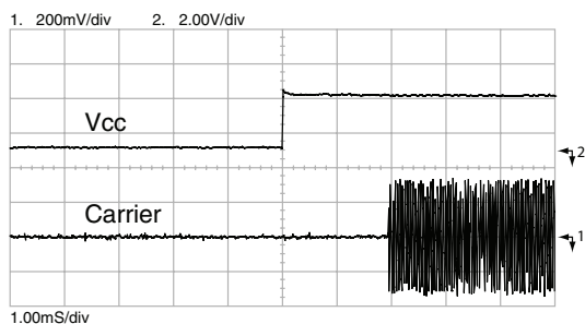
Figure 15: TX Turn-On Time from V cc
