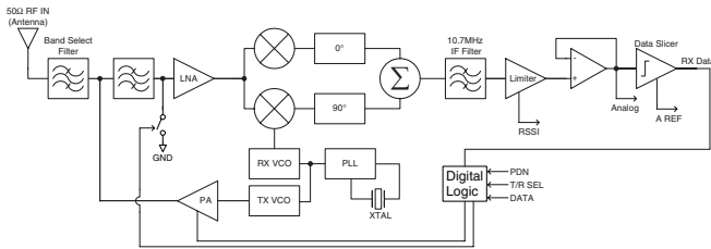
Figure 19: LT Series Transceiver Block Diagram
