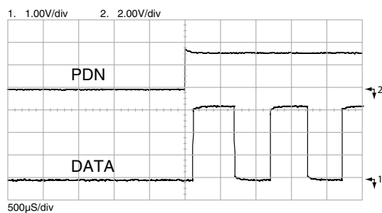
Figure 11: RX Turn-On Time from PDN
