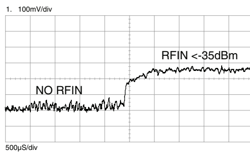
Figure 12: RSSI Response Time
