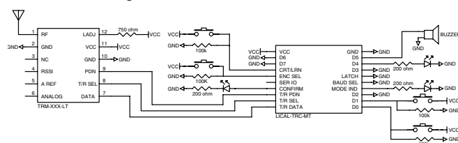
Figure 23: LT Series Transceiver and MT Series Transcoder
