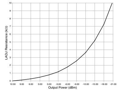
Figure 5: Output Power vs. LADJ Resistance
