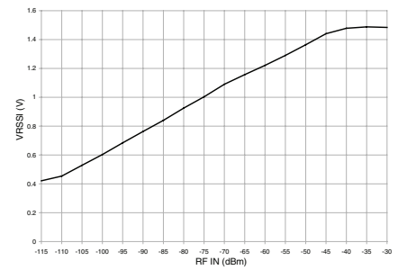
Figure 7: RSSI Curve
