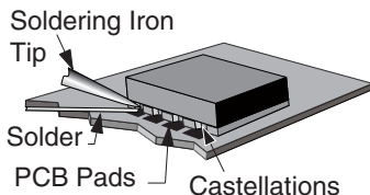
Figure 29: Soldering Technique
