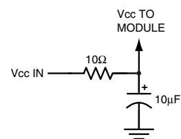
Figure 22: Supply Filter
