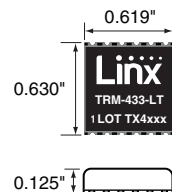
Figure 1: Package Dimensions
