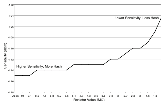
Figure 21: Sensitivity Degradation vs. Squelch Resistor
