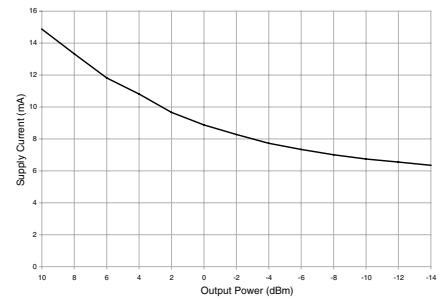
Figure 6: Output Power vs. Current Consumption
