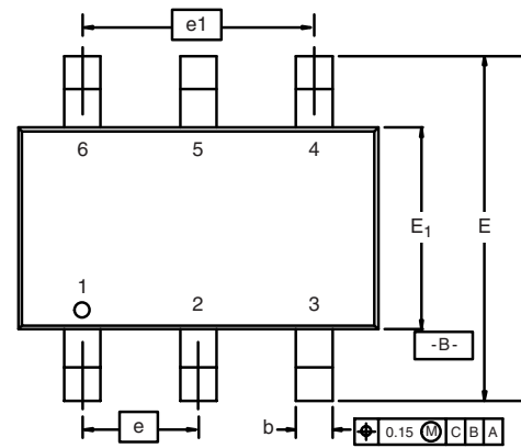
6-LEAD TSOP
