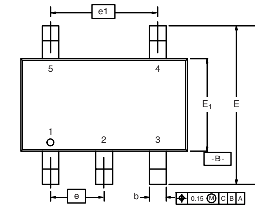
5-LEAD TSOP
