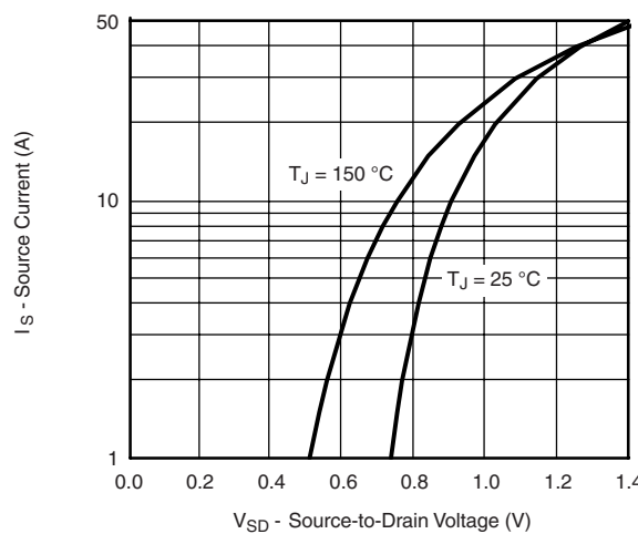
Source-Drain Diode Forward Characteristic
