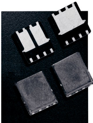
Fig. 1 PowerPAK 1212 Devices
