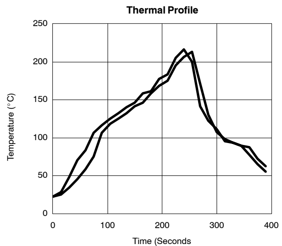
FIGURE 6. Reflow Profile
