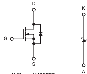
N-Channel MOSFET
