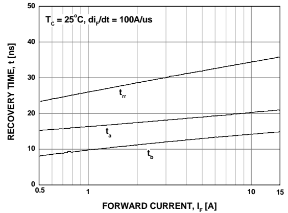
Figure 4. Recovery Time vs. Forward Current
