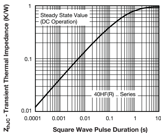
Fig. 13 - Thermal Impedance Z_{thJC} Characteristics
