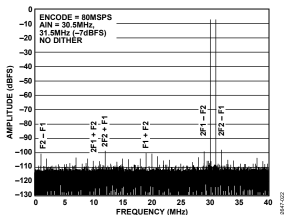
Figure 16. Two-Tone SFDR @ 30.5 MHz and 31.5 MHz
