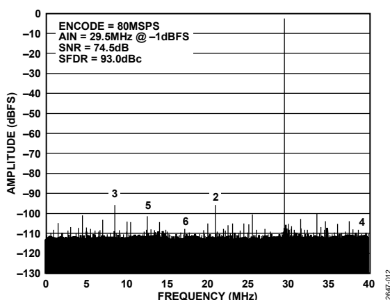
Figure 6. Single Tone @ 29.5 MHz
