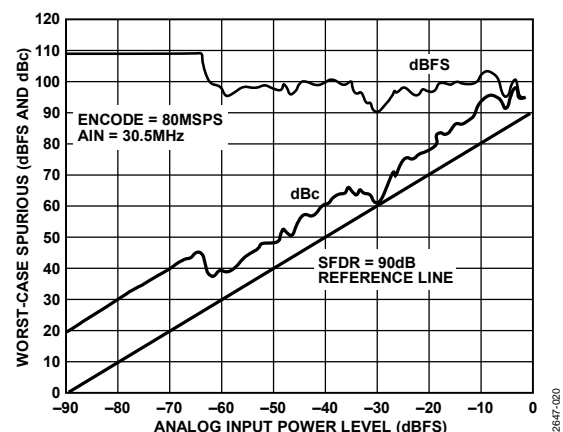
Figure 14. Single-Tone SFDR @ 30.5 MHz
