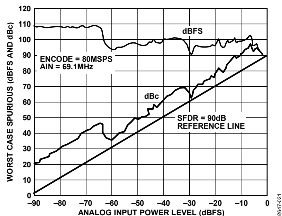
Figure 15. Single-Tone SFDR @ 69.1 MHz
