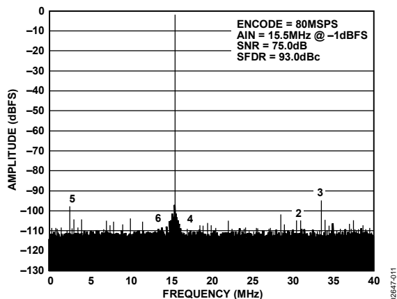
Figure 5. Single Tone @ 15.5 MHz
