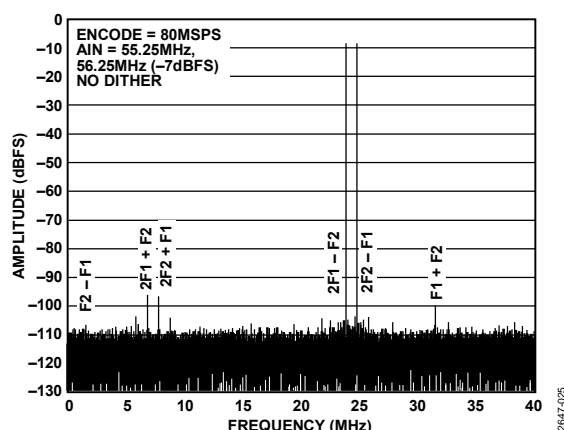
Figure 19. Two-Tone SFDR @ 55.25 MHz and 56.25 MHz
