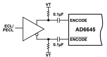
Figure 39. Differential ECL for Encode
