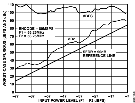
Figure 20. Two-Tone SFDR @ 55.25 MHz and 56.25 MHz
