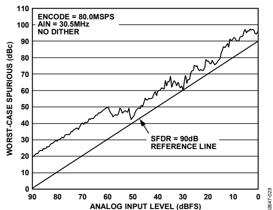
Figure 23. SFDR Without Dither
