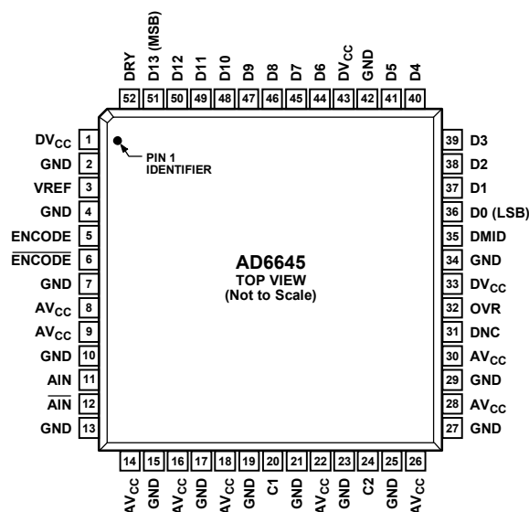
Figure 3. Pin Configuration
