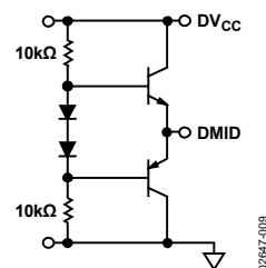
Figure 37. DMID Reference
