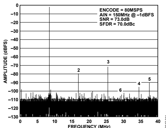
Figure 8. Single Tone @ 150 MHz
