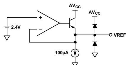
Figure 36. 2.4 V Reference
