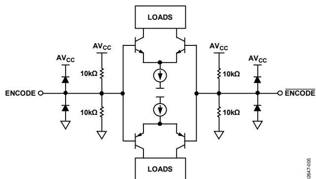
Figure 33. Encode Inputs
