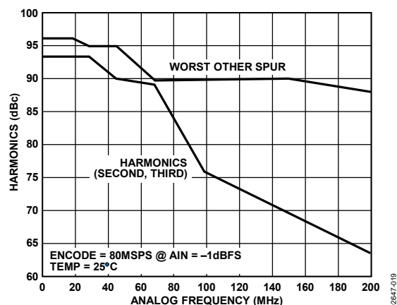
Figure 13. Harmonics vs. Analog Frequency (IF)
