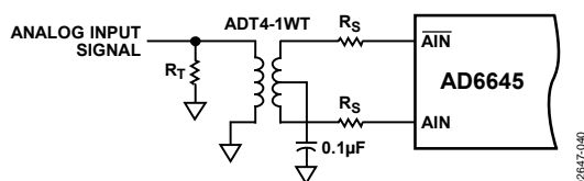
Figure 40. Transformer-Coupled Analog Input Circuit
