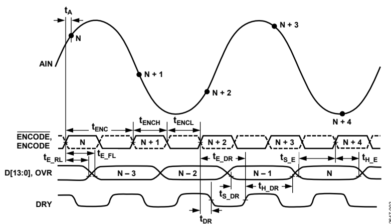
Figure 2. Timing Diagram
