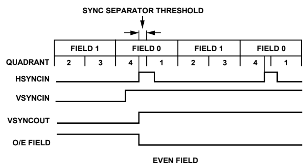
Figure 12. Vsync Filter—Even Field
