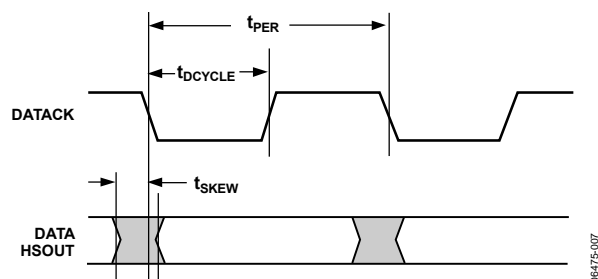
Figure 13. Output Timing
