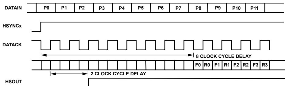
Figure 15. 4:2:2 Timing Mode
