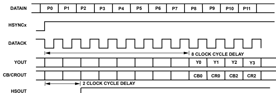
Figure 15. 4:2:2 Timing Mode
