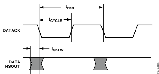
Figure 9. Output Timing
