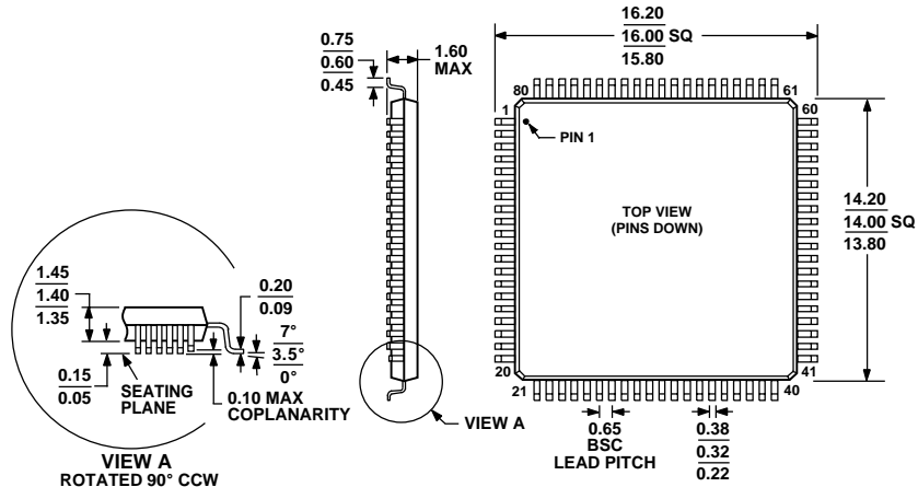
Figure 16. 80-Lead Low Profile Quad Flat Package [LQFP] (ST-80-2) Dimensions shown in millimeters
