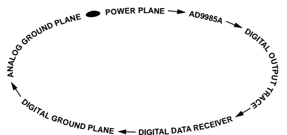
Figure 15. Current Loop
