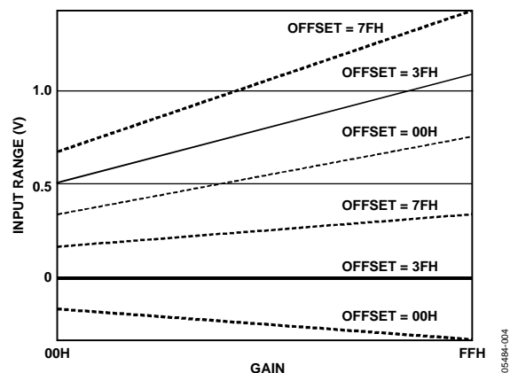
Figure 4. Gain and Offset Control
