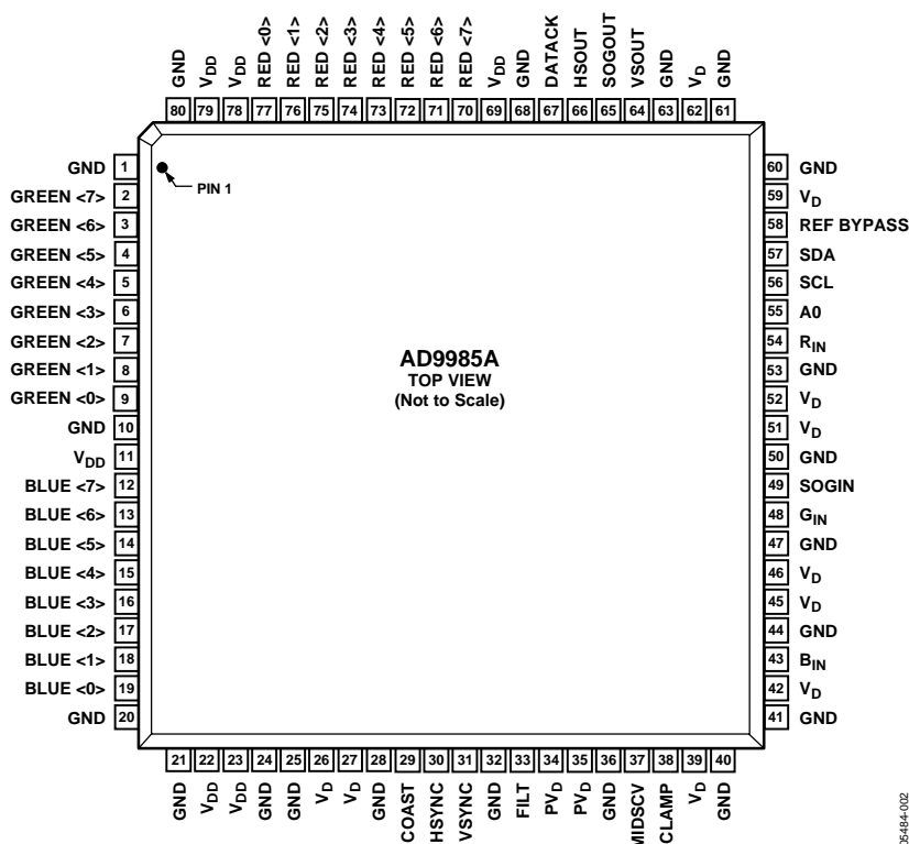
Figure 2. Pin Configuration
