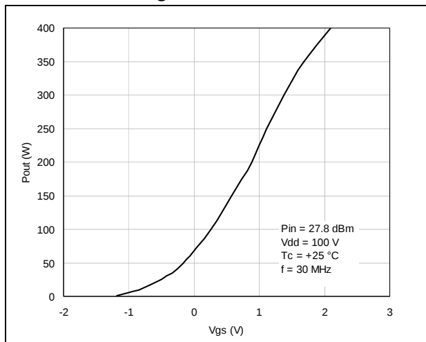
Figure 15. Output power vs. gate source voltage
