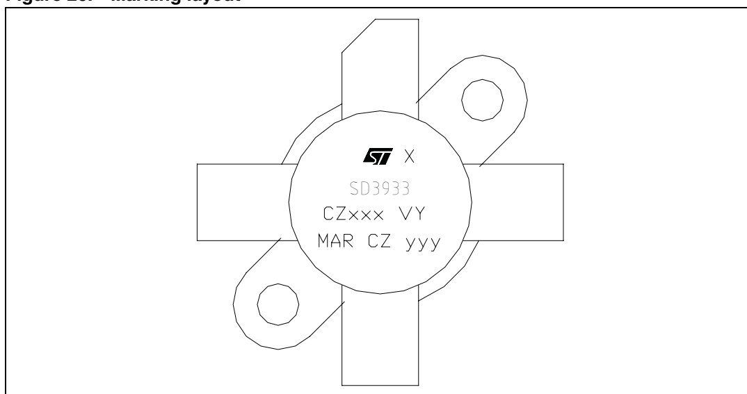
Figure 20. Marking layout
