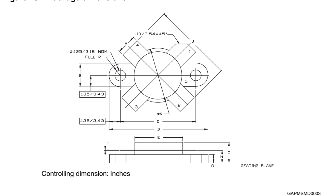
Figure 19. Package dimensions
