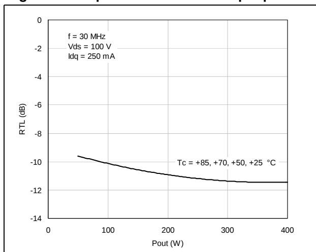
Figure 13. Input return loss vs. output power
