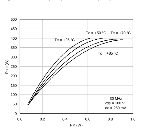
Figure 8. Output power vs. input power
