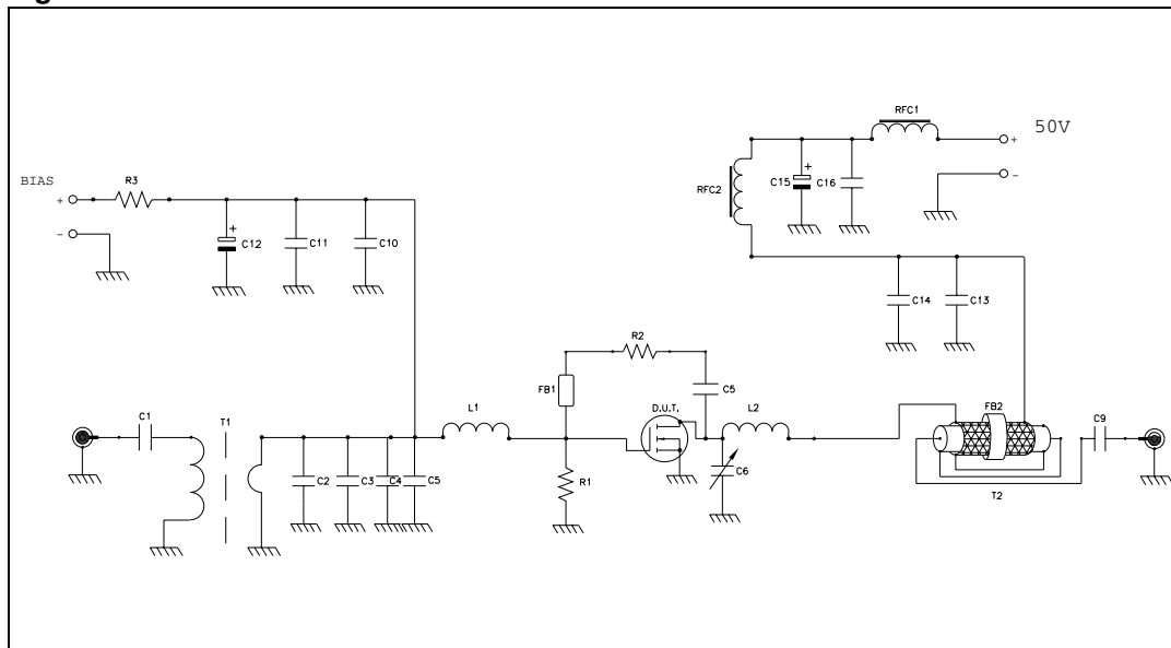
Figure 16. Test circuit
