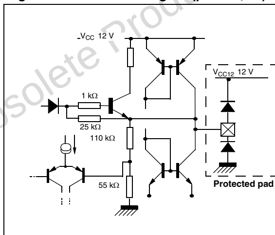
Figure 14. Slow blanking I/O (pins 59, 61)
