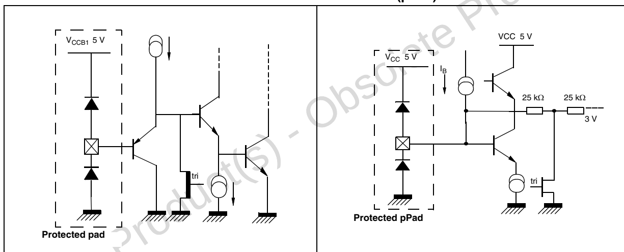
Figure 9. Average clamped video inputs (pin 8)
