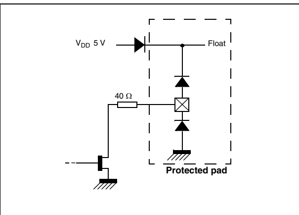
Figure 19. I 2 C bus (ADD) (pin 54)
