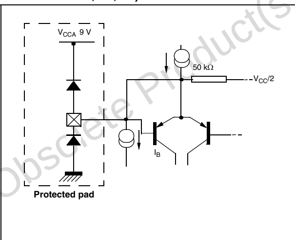
Figure 13. Audio inputs (pins 7, 9 11, 13, 19, 20, 22, 23)
