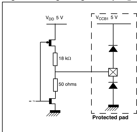
Figure 10. C gate logical output (pin 52)
