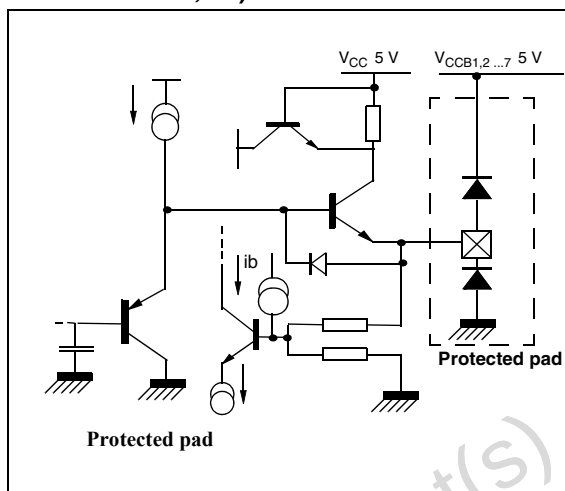
Figure 12. Video outputs (pins 38, 40, 42, 44, 46, 48)
