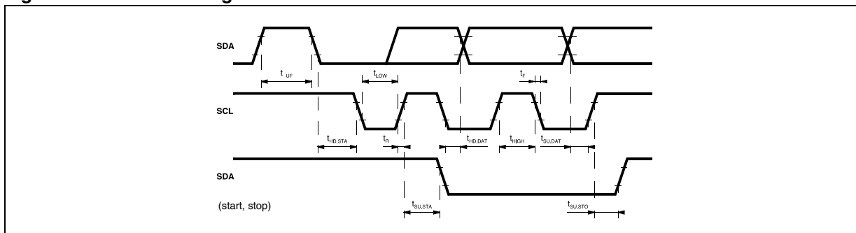
Figure 4. I 2 C bus timing
