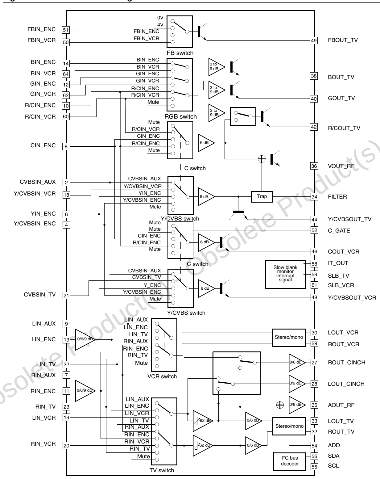
Figure 2. STV6412A block diagram
