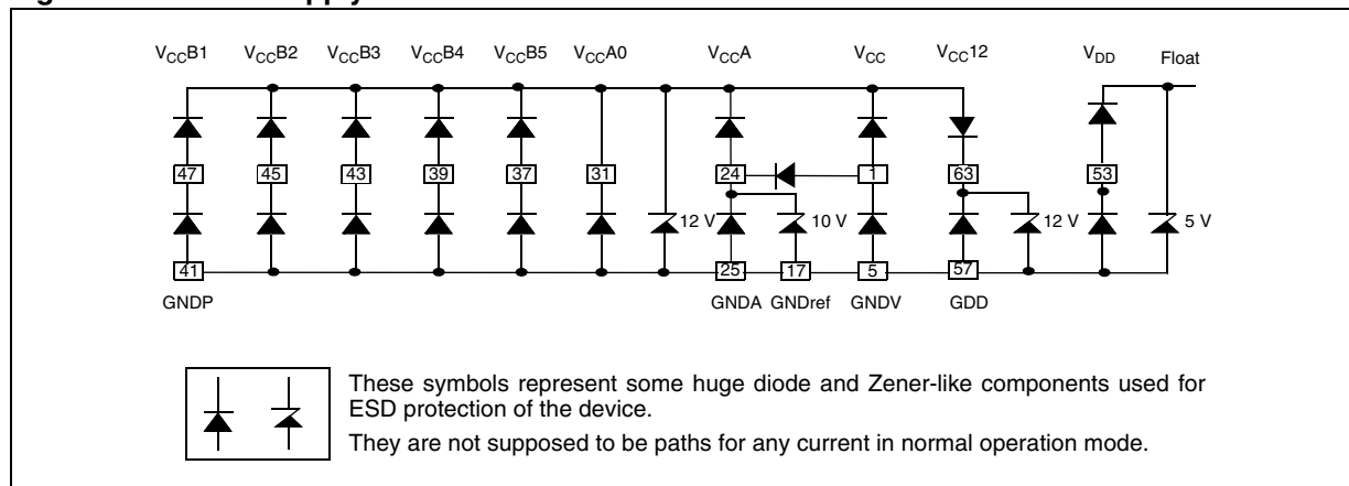
Figure 21. Power supply connection
