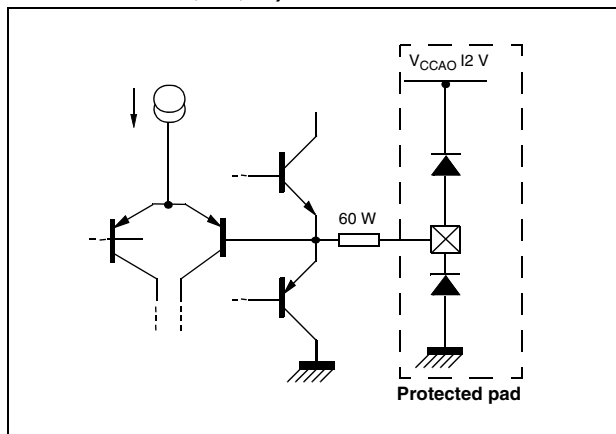
Figure 16. Audio outputs (pins 27, 28, 29, 30, 32, 33, 35)
