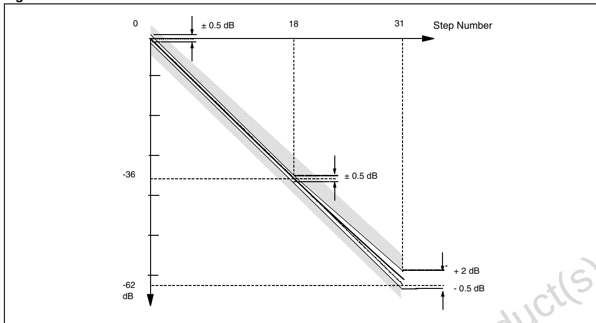
Figure 5. Volume control characteristics
