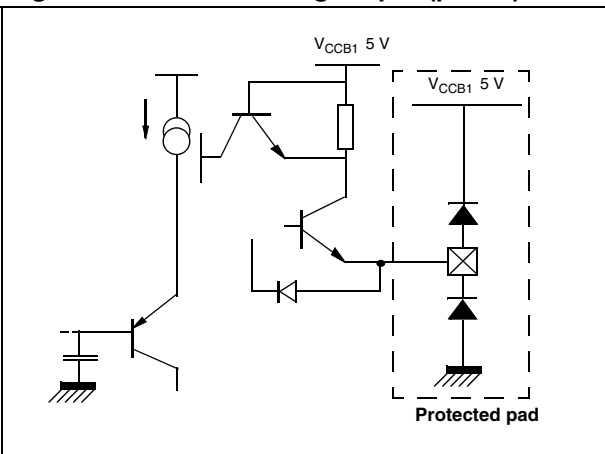
Figure 11. Fast blanking output (pin 49)
