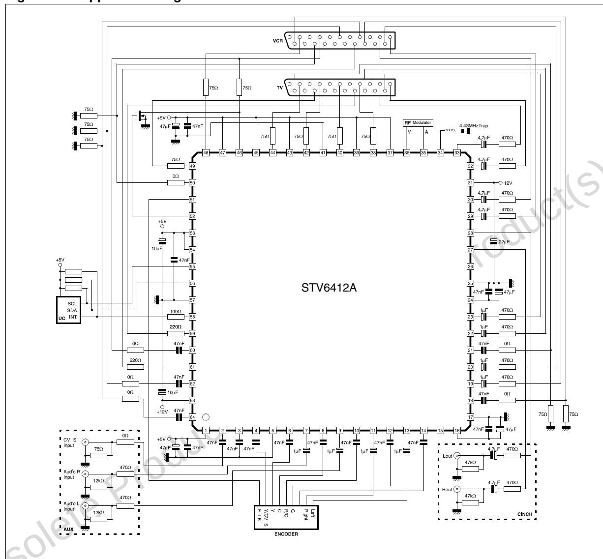
Figure 22. Application diagram
