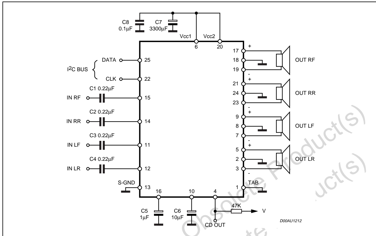
Figure 1. Application Circuit
