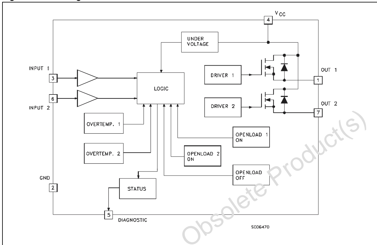
Figure 2. Block Diagram
