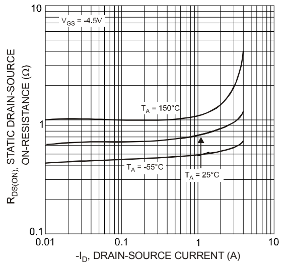
Fig. 14 Static Drain-Source On-Resistance vs. Drain Current
