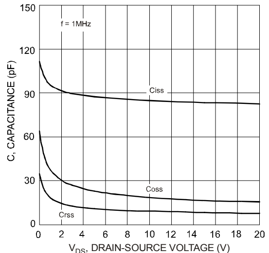
Fig. 10 Typical Capacitance
