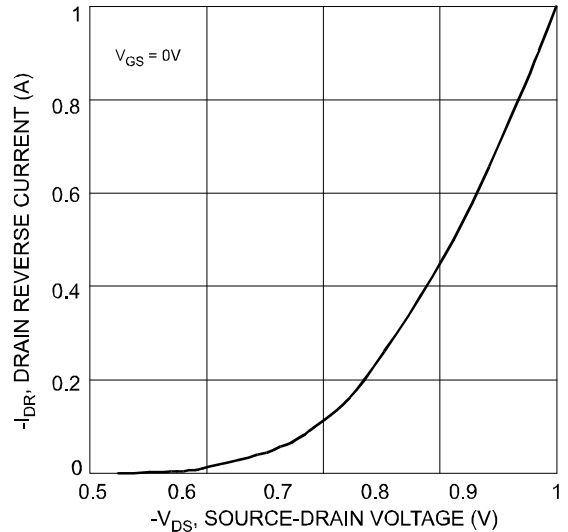
Fig. 18 Drain Reverse Current vs. Source-Drain Voltage
