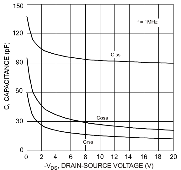
Fig. 20 Typical Capacitance
