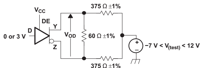
Figure 11. Driver V_{OD} With Common-Mode Loading Test Circuit
