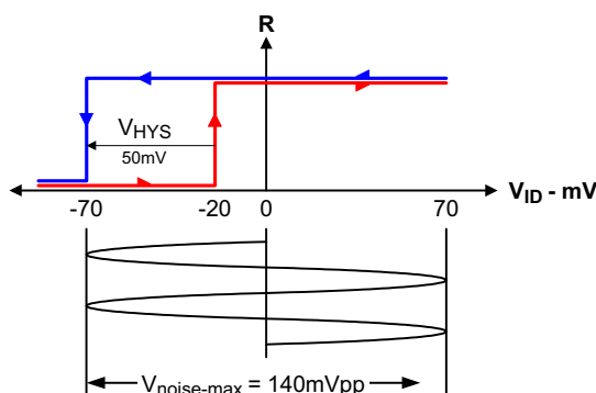
Figure 23. SN65HVD30-35 Noise Immunity Under Bus Fault Conditions
