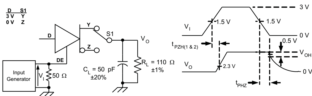
Figure 14. Driver Switching Test Circuit and Voltage Waveforms
