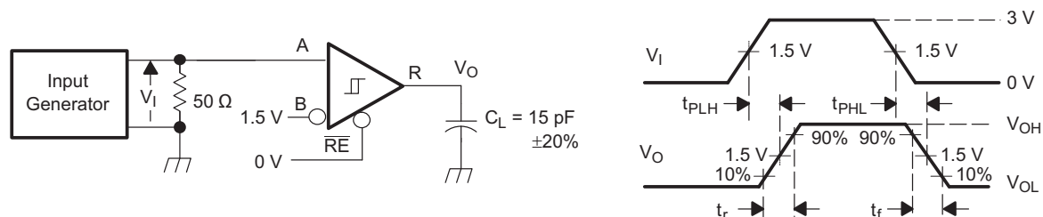
Figure 18. Receiver Switching Test Circuit and Voltage Waveforms
