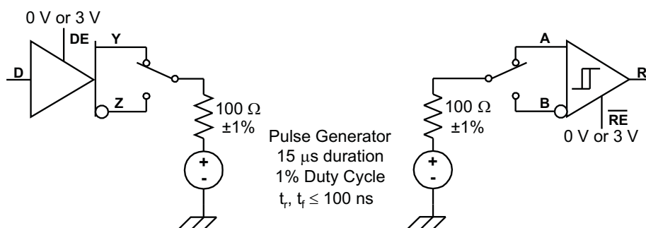
Figure 21. Test Circuit, Transient Over Voltage Test
