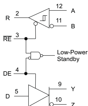
Figure 22. Low-Power Standby Logic Diagram
