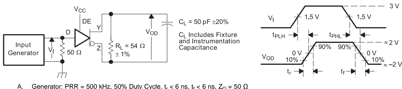
Figure 14. Driver Switching Test Circuit and Voltage Waveforms
