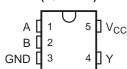
DBV OR DCK PACKAGE (TOP VIEW)
