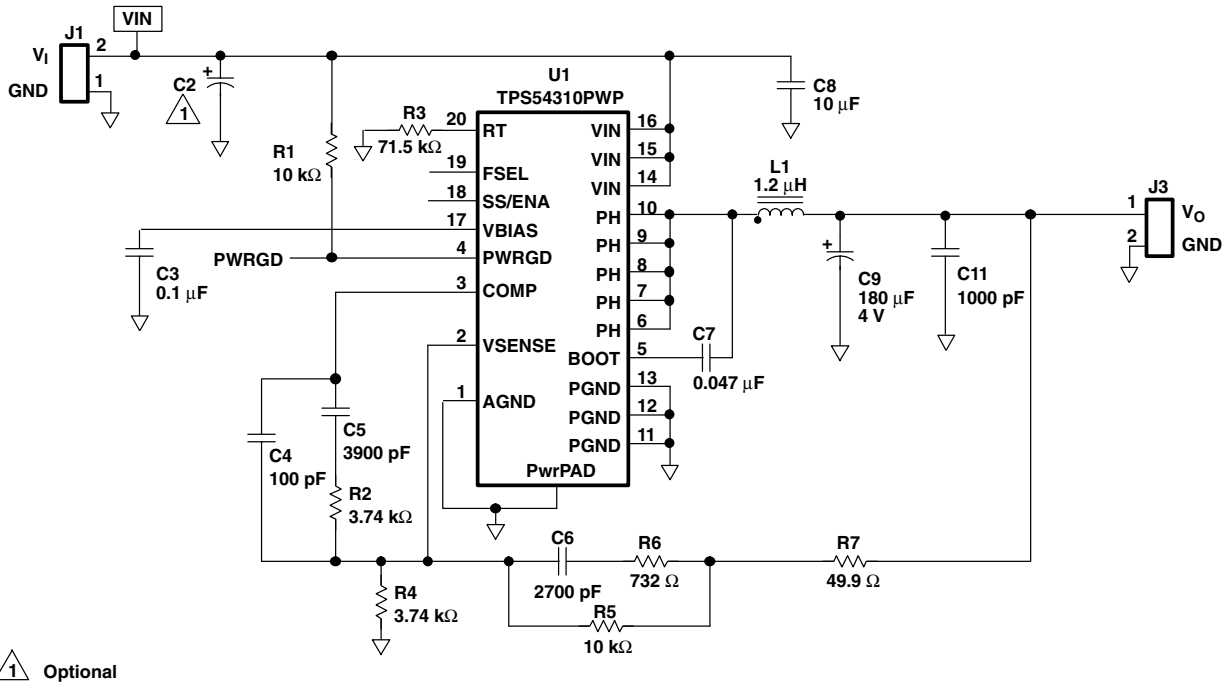
Figure 10. TPS54310 Schematic
