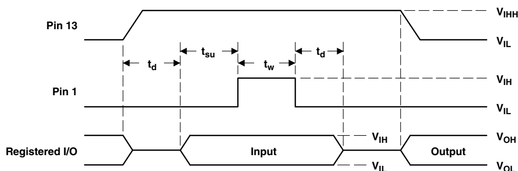
Figure 2. Preload Waveforms
