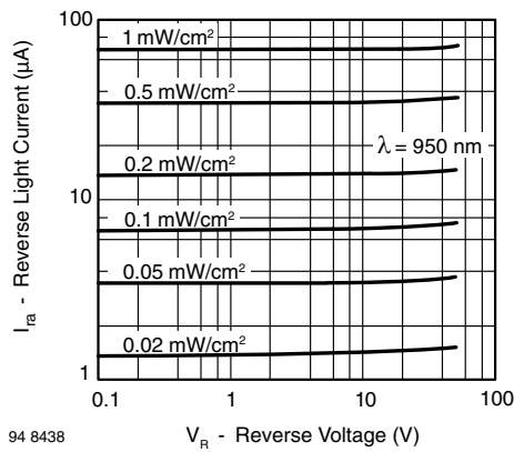
94 8438 Fig. 4 - Reverse Light Current vs. Reverse Voltage
