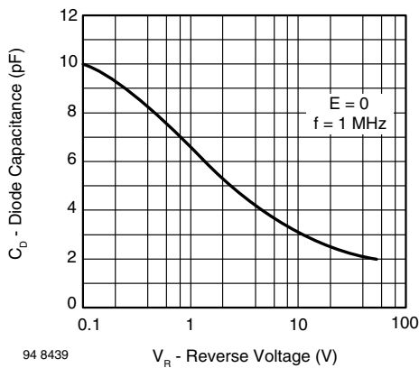
94 8439 Fig. 5 - Diode Capacitance vs. Reverse Voltage
