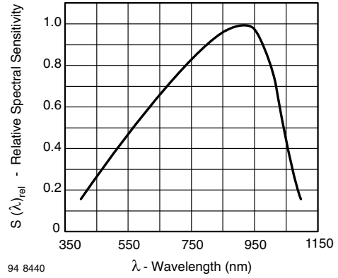
94 8440 Fig. 6 - Relative Spectral Sensitivity vs. Wavelength
