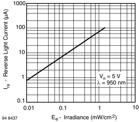
94 8437 Fig. 3 - Reverse Light Current vs. Irradiance
