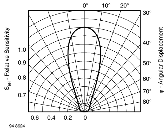
94 8624 Fig. 7 - Relative Radiant Sensitivity vs. Angular Displacement
