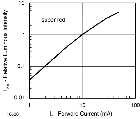
Figure 9. Relative Luminous Intensity vs. Forward Current
