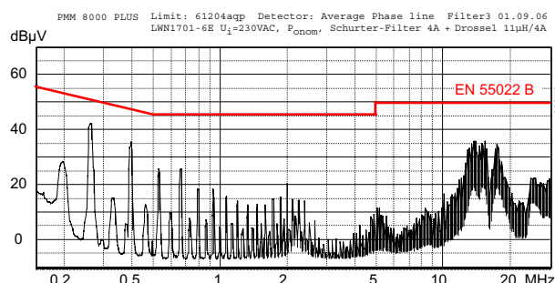
Fig. 14b Conducted disturbances (average) of LW models (feature E) with external filter at phase input according to EN 55011/ 55022, at V_i = 230\text{ VAC} , I_{o\text{ nom}} (LWN1701-6E).
