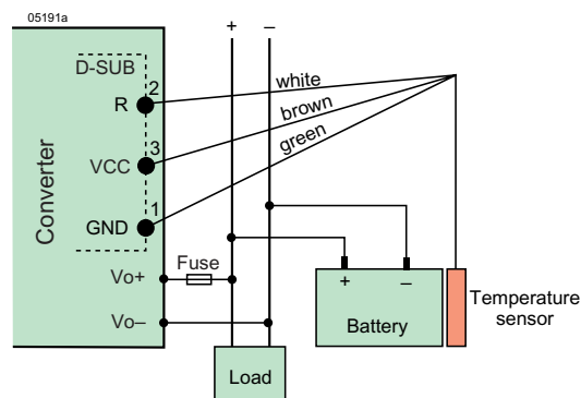
Fig. 30 Connection of temperature sensor
