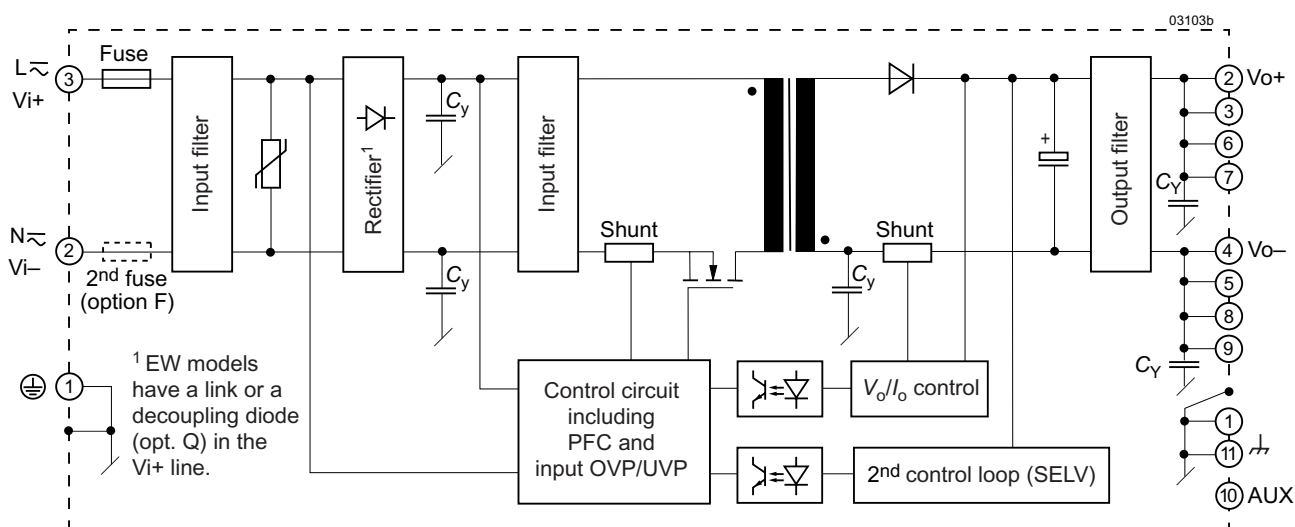
Fig. 1 Single-output converters (125 W).
