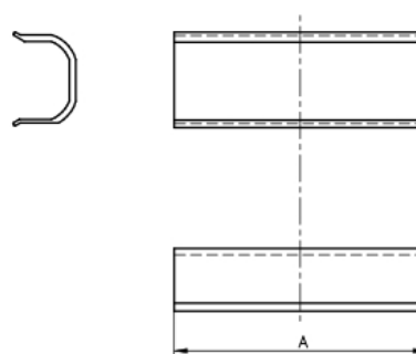
Fig. 28 Protective covers HZZ01219-G
