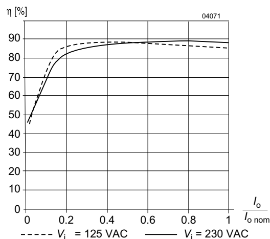
Fig. 3 Efficiency versus load (LWN2660-6)
