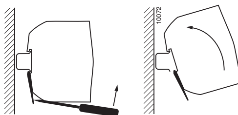
Fig. 18b Dismounting from DIN-rail. Use proper tool (min. 3 mm screwdriver) and adequate force.
