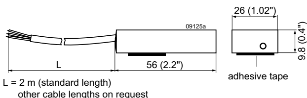
Fig. 29 Temperature sensor
