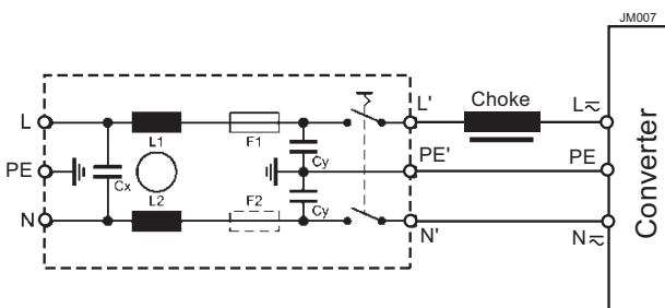
Fig. 15a External filter to reduce conducted emissions of LW models with feature E ( L_1 = L_2 = 1.6\text{ mH} , C_x = 47\text{ nF} , C_y = 2.2\text{ nF} )
