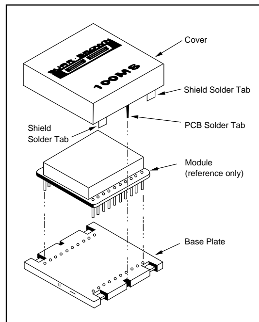
FIGURE 2. Assembly Diagram.
