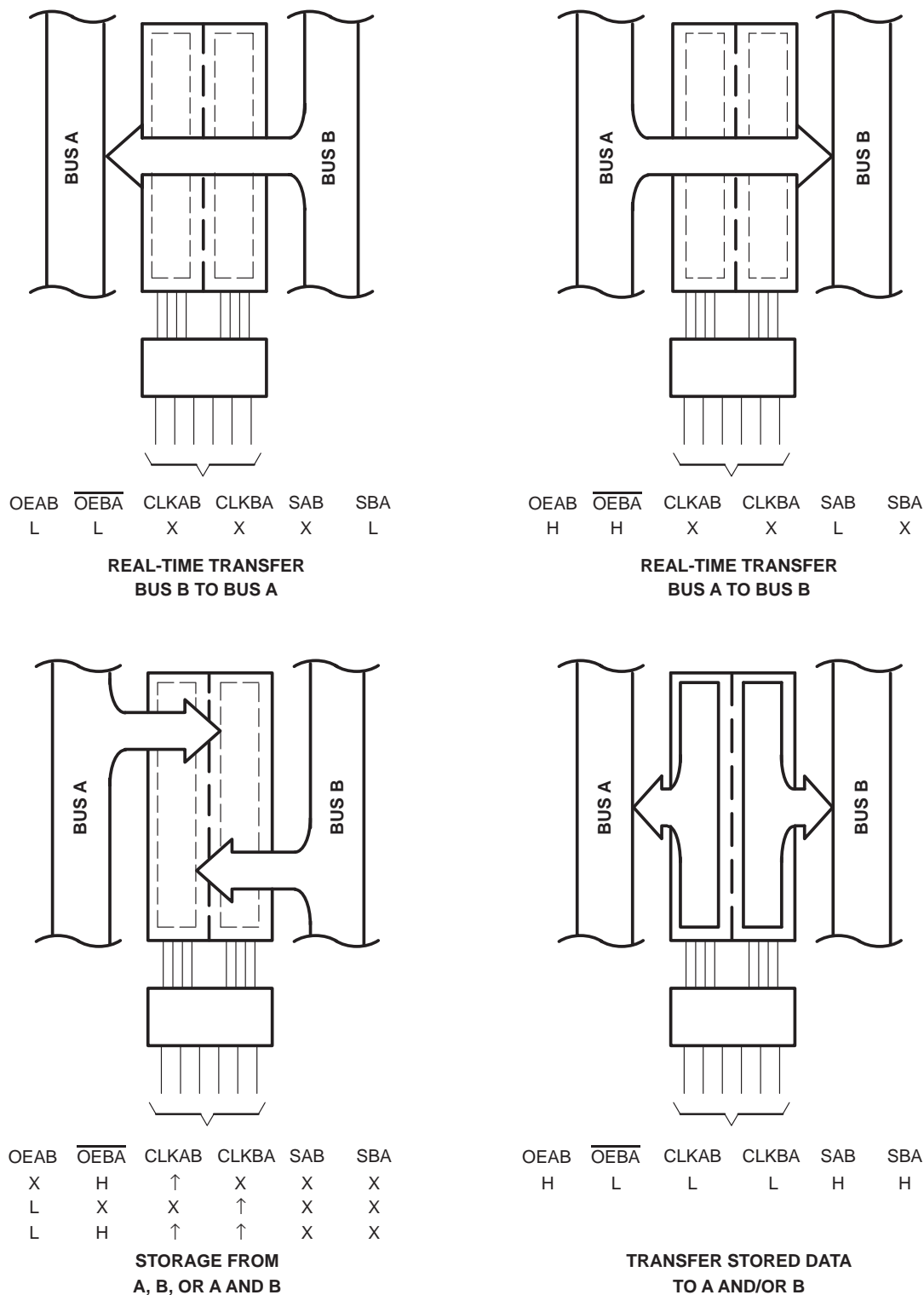
Figure 1. Bus-Management Functions
