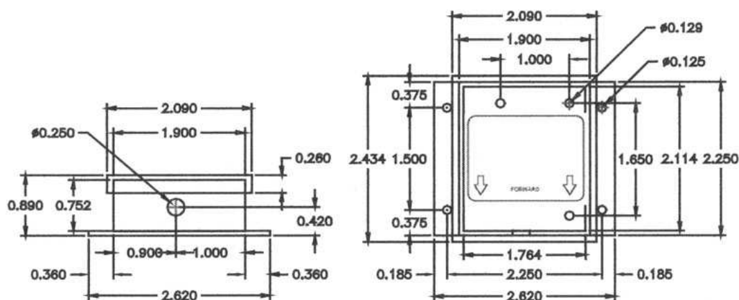
Figure 2 HMR3500 Case Dimensions
