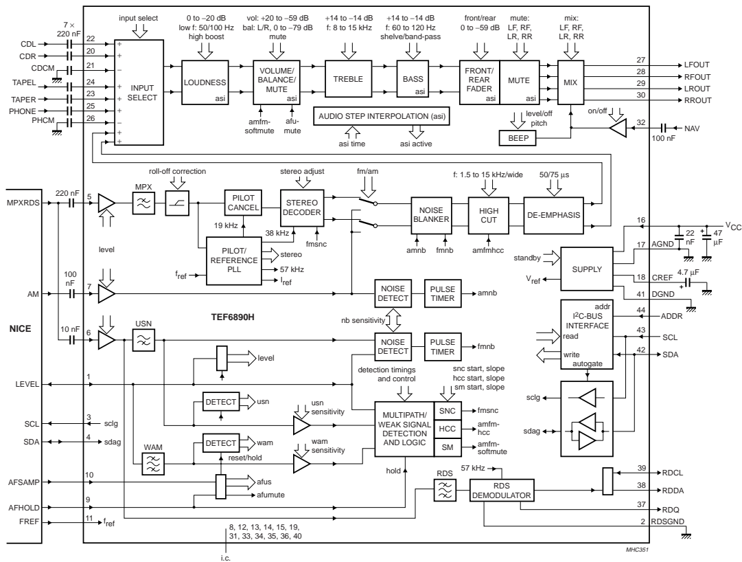
Fig.24 Application diagram.
