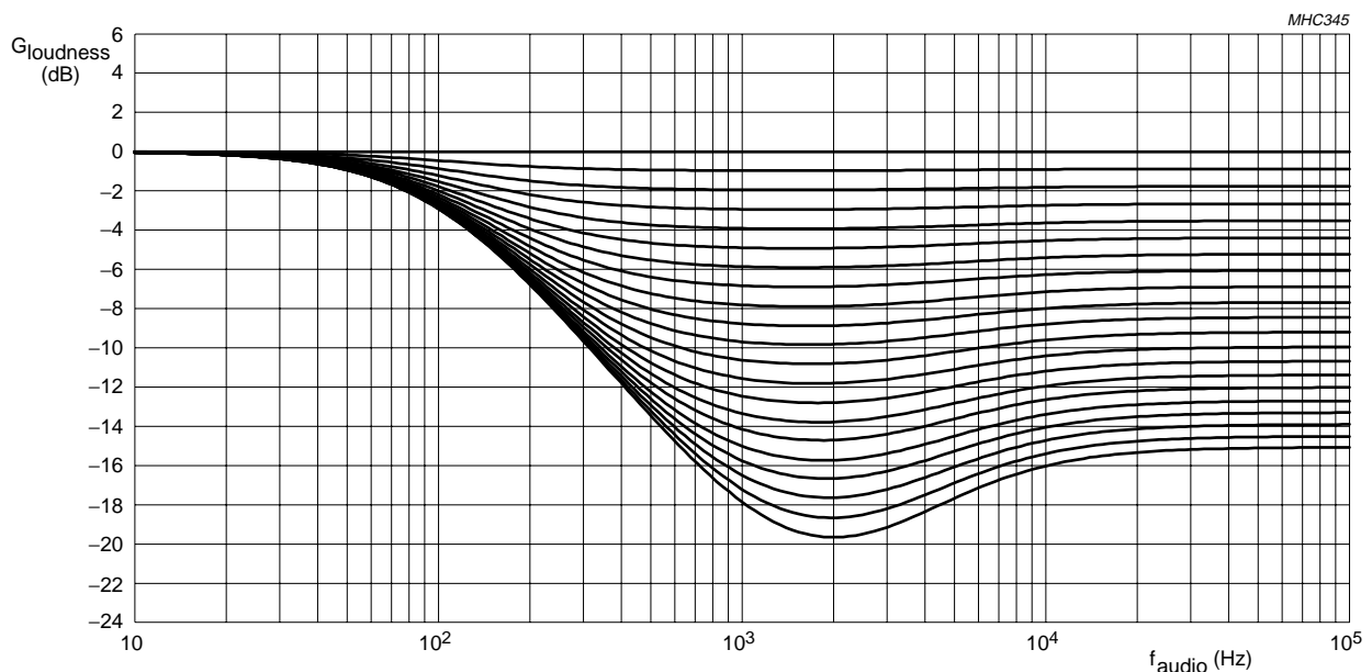
Fig.18 Loudness gain G_{\text{loudness}} as a function of audio frequency f_{\text{audio}} ; low boost frequency 100 Hz and high boost on.
