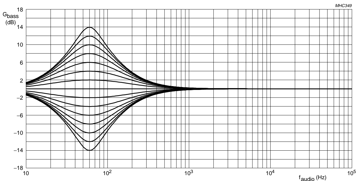
Fig.22 Bass gain G_{\text{bass}} as a function of audio frequency f_{\text{audio}} ; bass frequency 60 Hz, band-pass boost and band-pass cut.
