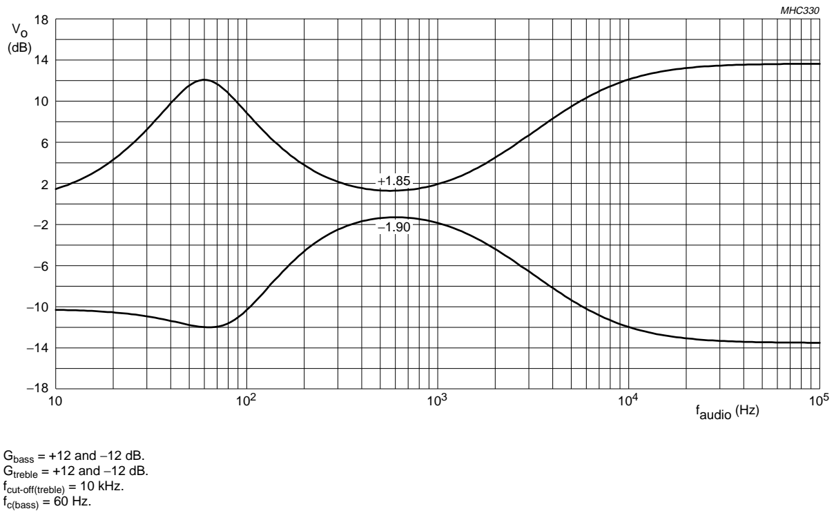
Fig.3 Equalizer bowing.
