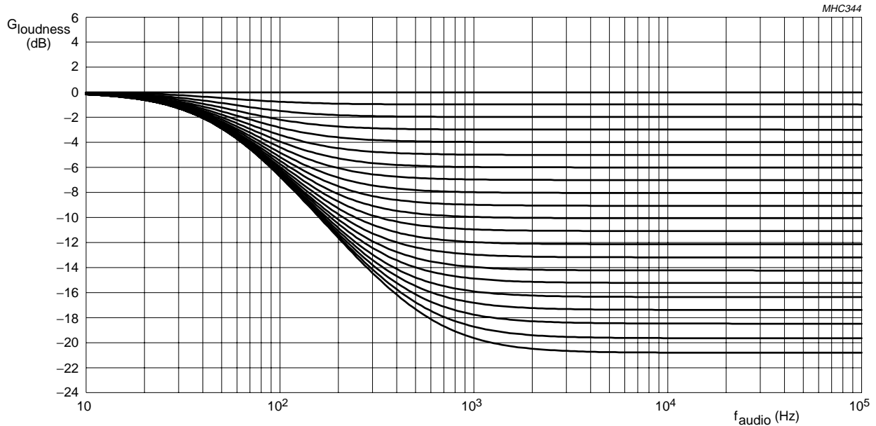
Fig.17 Loudness gain G_{\text{loudness}} as a function of audio frequency f_{\text{audio}} ; low boost frequency 50 Hz and high boost off.
