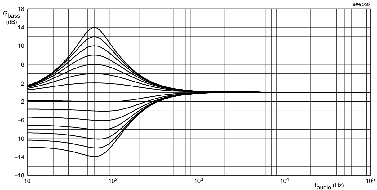
Fig.21 Bass gain G_{\text{bass}} as a function of audio frequency f_{\text{audio}} ; bass frequency 60 Hz, band-pass boost and shelve cut.
