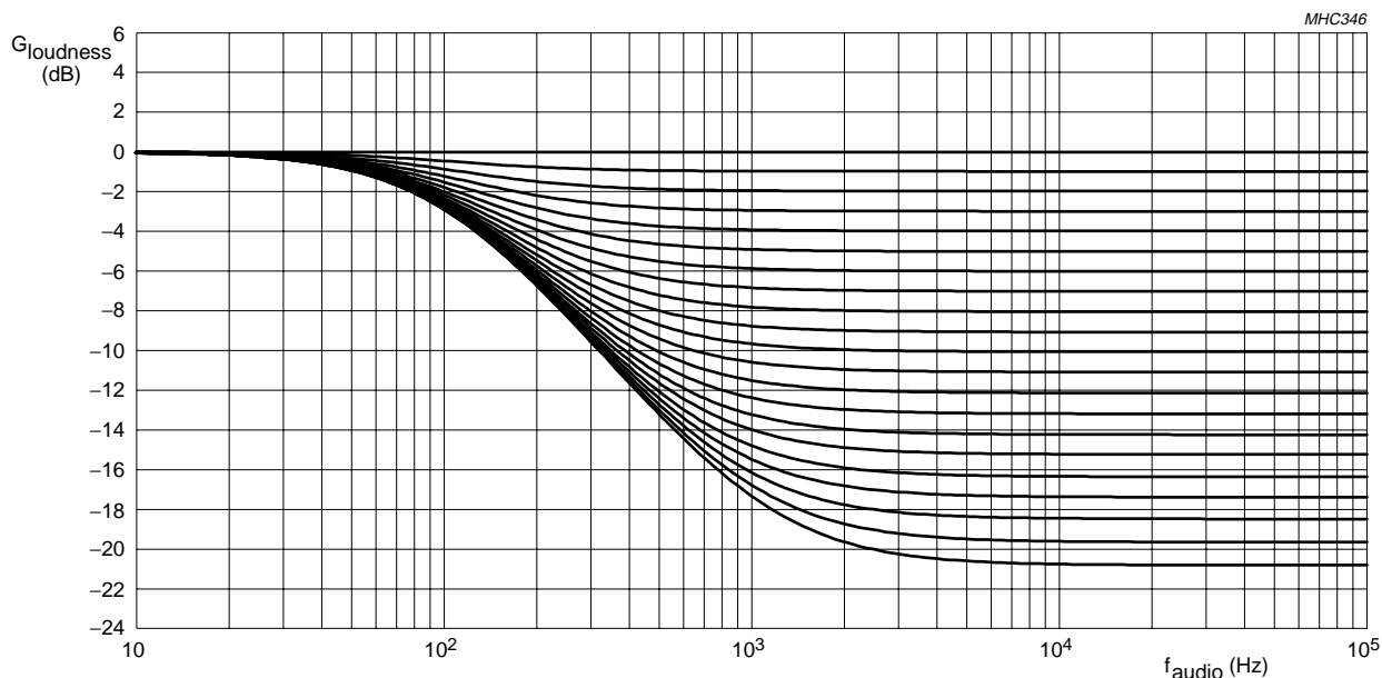
Fig.19 Loudness gain G_{\text{loudness}} as a function of audio frequency f_{\text{audio}} ; low boost frequency 100 Hz and high boost off.
