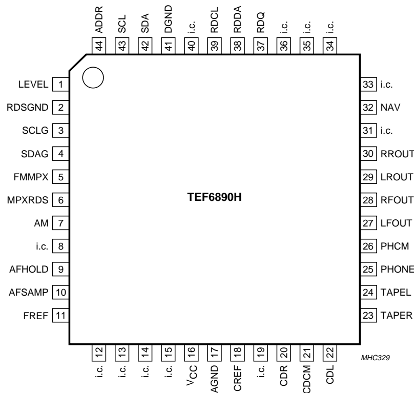
Fig.2 Pin configuration.
