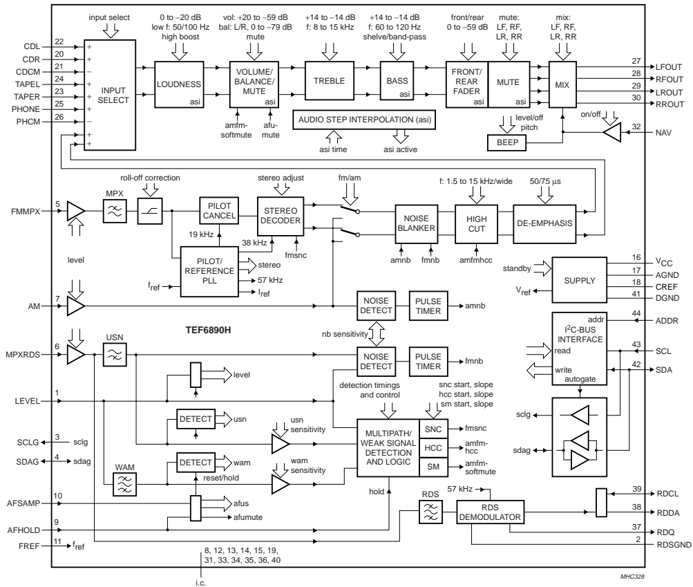
Fig.1 Block diagram.
