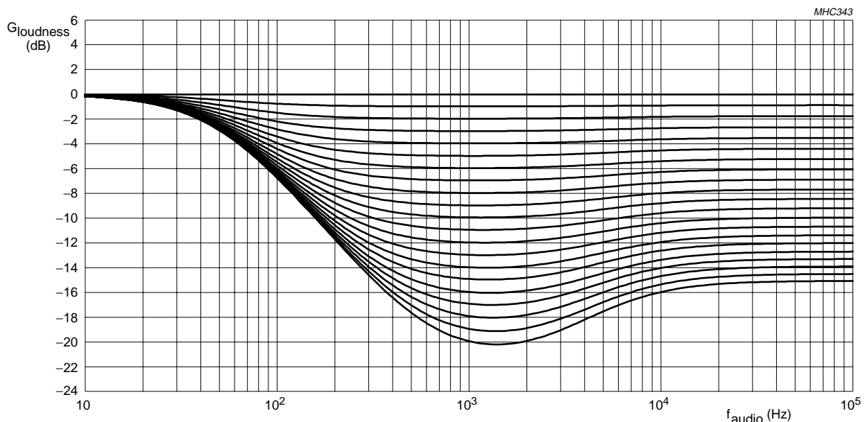
Fig.16 Loudness gain G_{\text{loudness}} as a function of audio frequency f_{\text{audio}} ; low boost frequency 50 Hz and high boost on.
