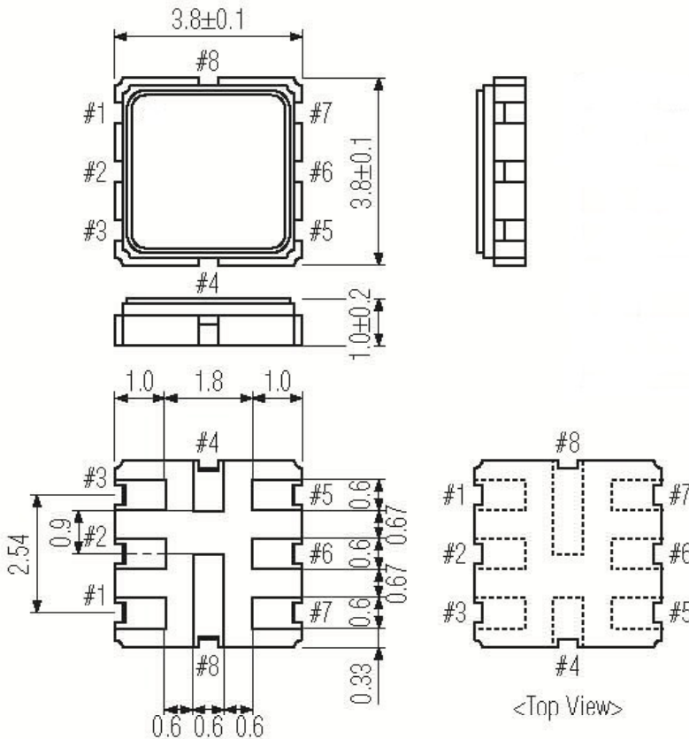
Figure 1) Top, Side and Bottom Views
