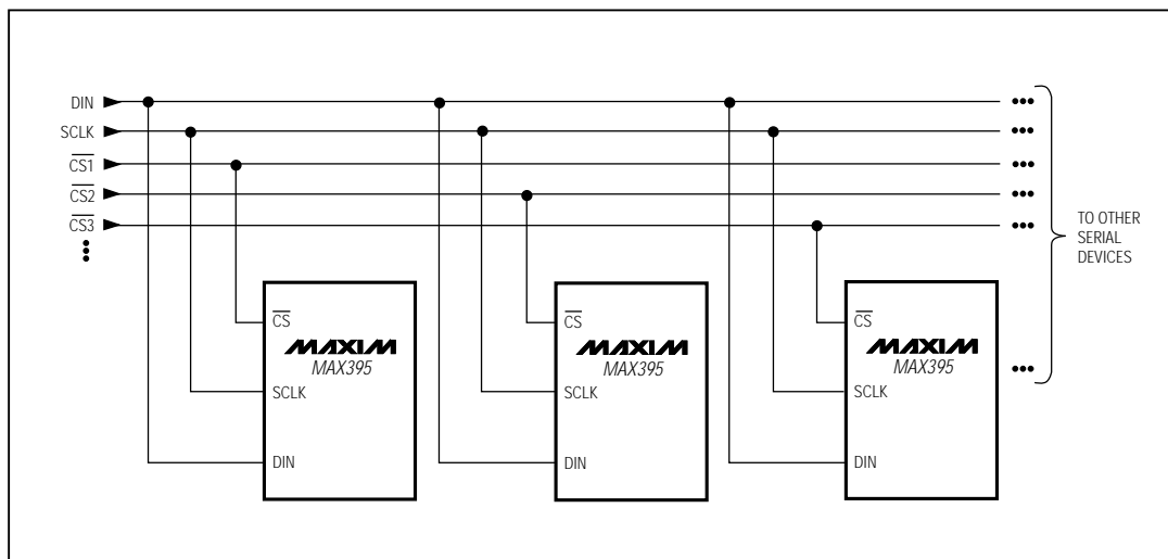
Figure 6. Addressable Serial Interface
