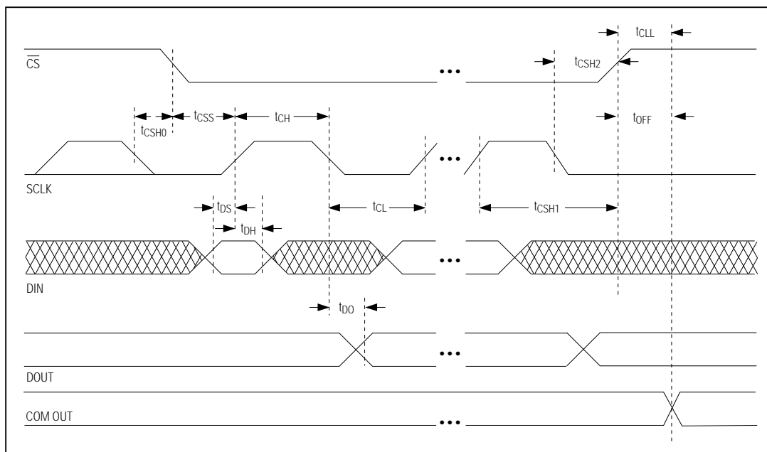
Figure 1. Timing Diagram
