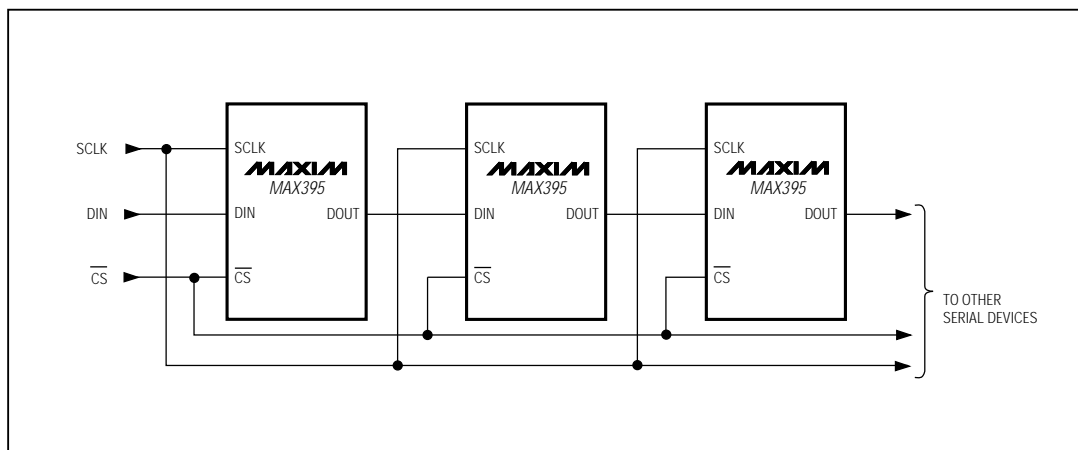
Figure 5. Daisy-Chained Connection
