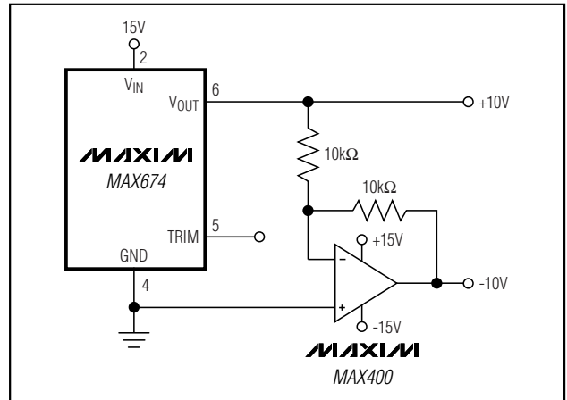
Figure 3. ±10V Reference
