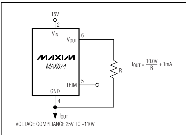
Figure 4. Current Source
