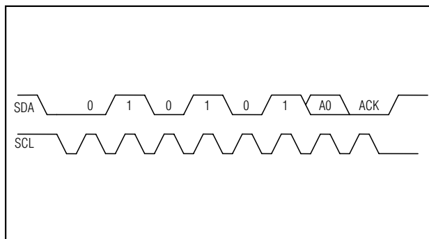
Figure 9. Slave Address
