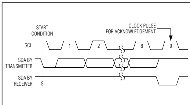
Figure 8. Acknowledge
