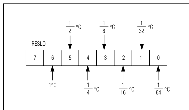
Figure 1. Temperature Measured in 1/64°C Steps
