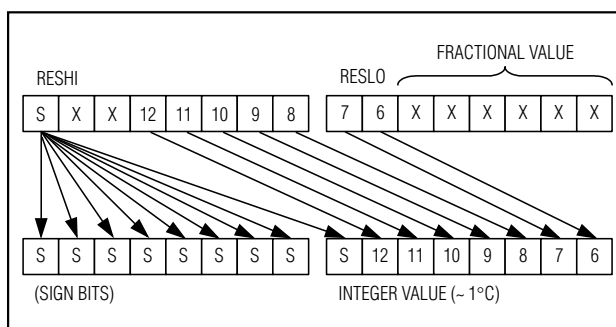
Figure 3. Alternate Temperature Representation
