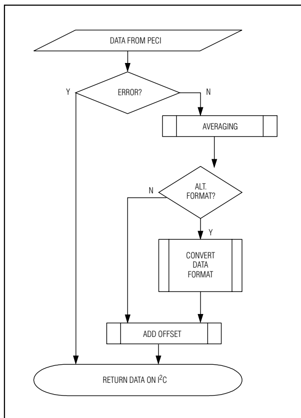
Figure 4. Operational Flowchart
