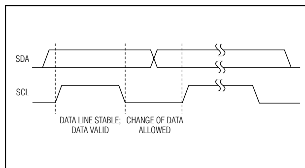
Figure 7. Bit Transfer
