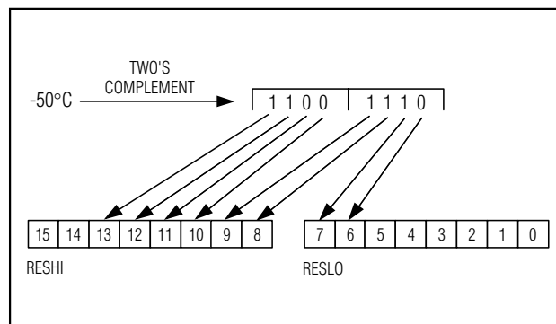
Figure 2. Conversion of Temperature Done in Two's Complement
