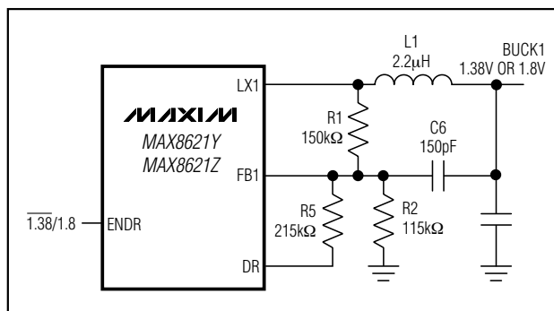
Figure 1. Adjusting BUCK1 Output Voltage Using DR
