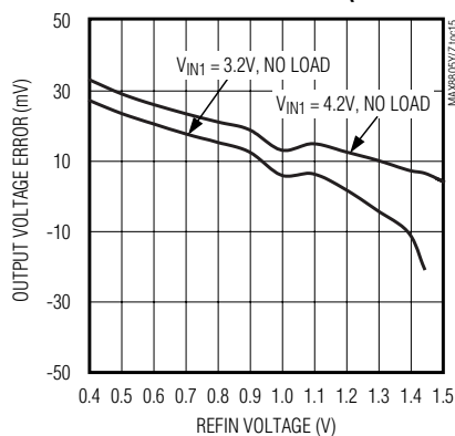
REFIN vs. REFIN TO OUT GAIN (MAX8805Y)
