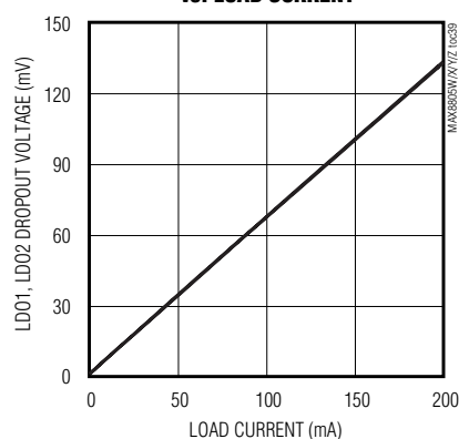
LD01, LD02 DROPOUT VOLTAGE vs. LOAD CURRENT
