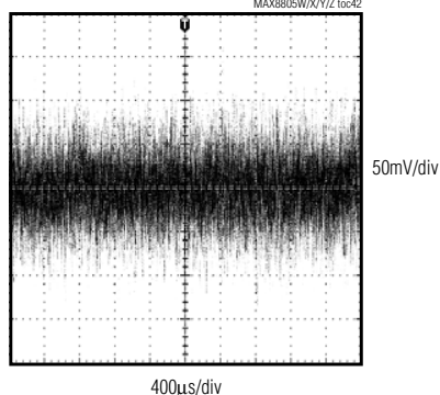
LD01, LD02 OUTPUT NOISE WAVEFORM
