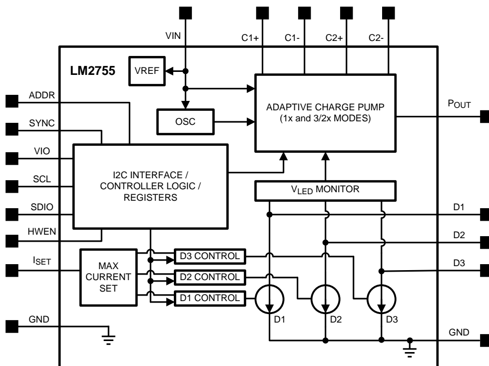
Figure 16. Block Diagram
