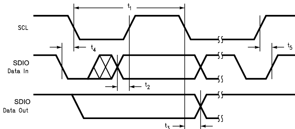
Figure 4. I²C Timing Diagram
