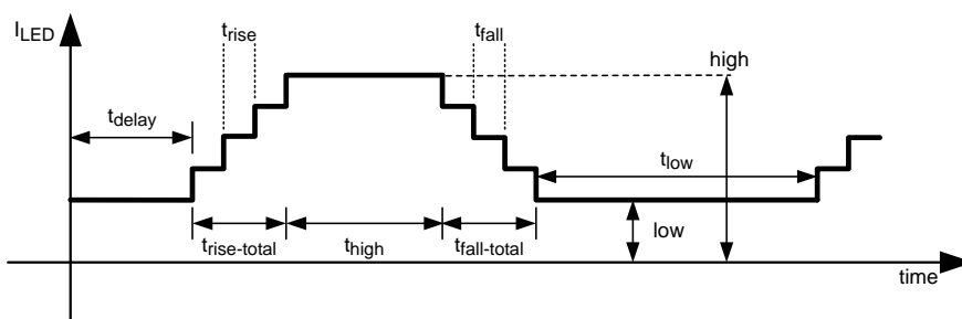
Figure 20. Dimming Waveform
