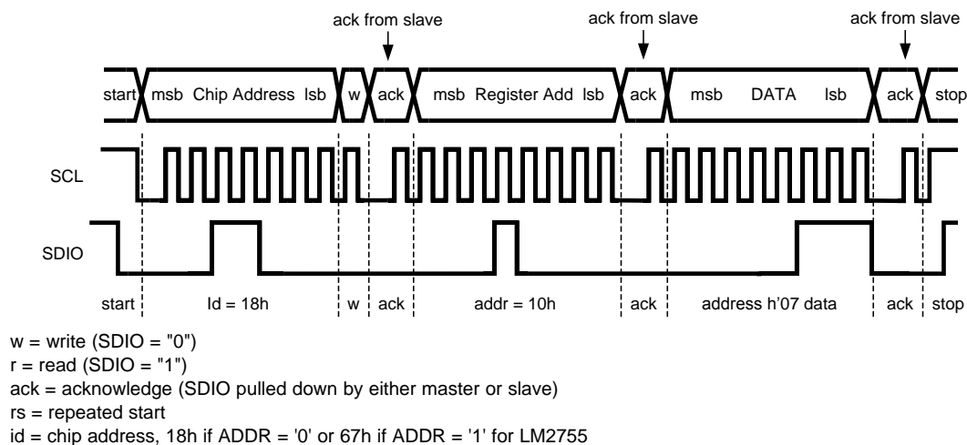
Figure 19. Write Cycle
