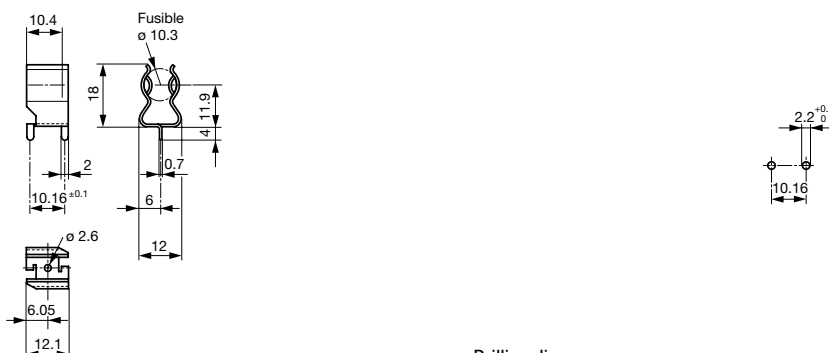
Drilling diagram
