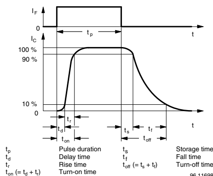
Fig. 4 - Switching Times
