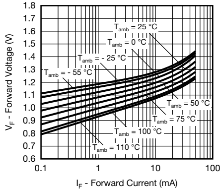
Fig. 5 - Forward Voltage vs. Forward Current
