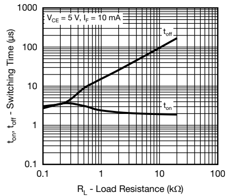
Fig. 15 - Switching Time vs. Load Resistance
