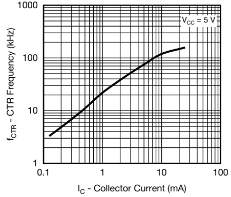
Fig. 14 - CTR -3 dB Frequency vs. Collector Current
