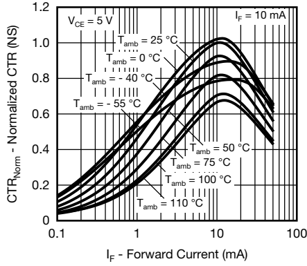
Fig. 11 - Normalized CTR (NS) vs. Forward Current
