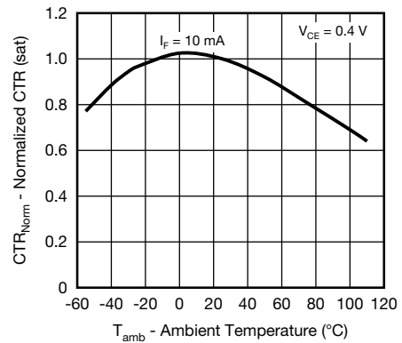
Fig. 10 - Normalized CTR (sat) vs. Ambient Temperature
