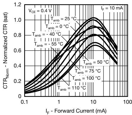
Fig. 12 - Normalized CTR (sat) vs. Forward Current
