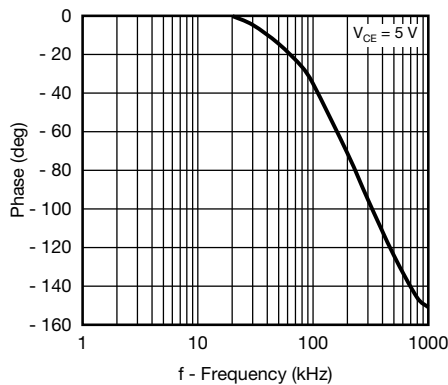
Fig. 13 - CTR Frequency vs. Phase Angle
