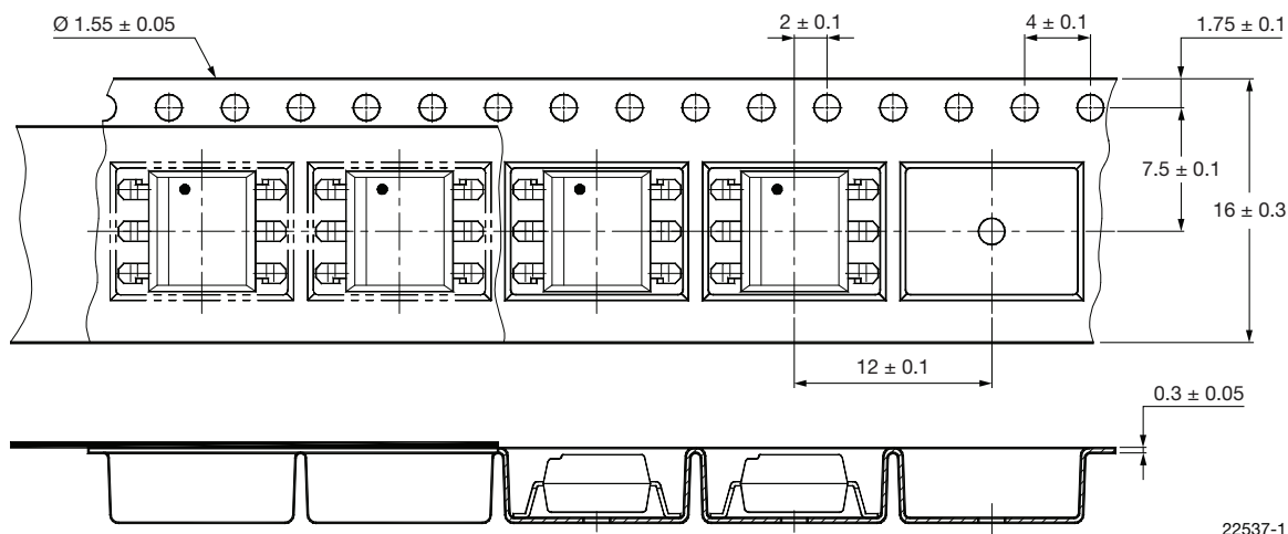
Fig. 16 - Tape and Reel Drawing, 1000 Units per Reel
