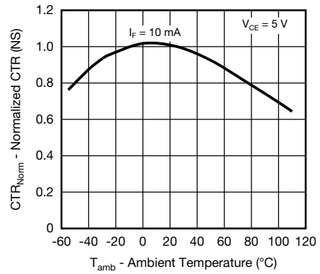
Fig. 9 - Normalized CTR (NS) vs. Ambient Temperature
