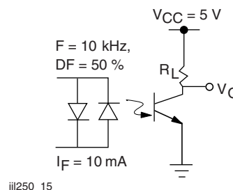
Fig. 15 - Switching Schematic
