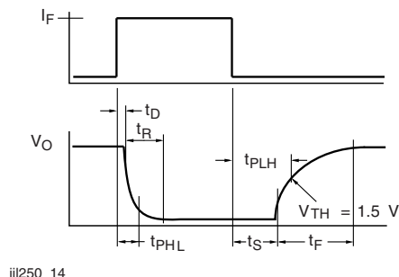
Fig. 14 - Switching Timing
