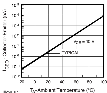
Fig. 7 - Collector Emitter Leakage Current vs. Temperature
