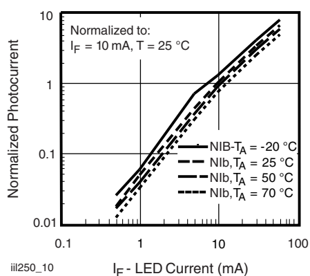
Fig. 10 - Normalized Photocurrent vs. I_F and Temperature
