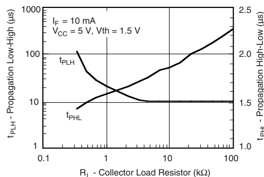
Fig. 10 - Propagation Delay vs. Collector Load Resistor
