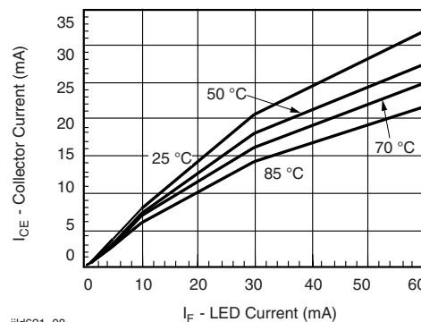
Fig. 8 - Collector Emitter Current vs. Temperature and LED Current
