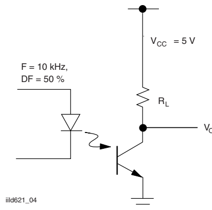
Fig. 4 - Saturated Switching Timing
