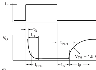
Fig. 3 - Saturated Switching Timing
