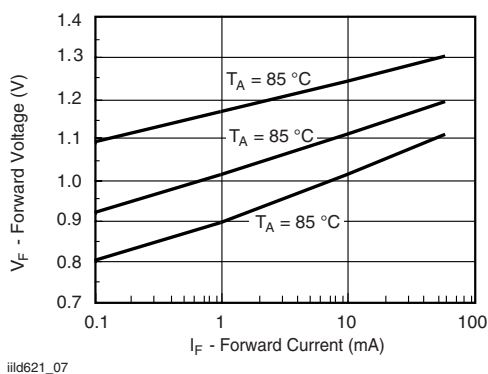
Fig. 7 - Forward Voltage vs. Forward Current
