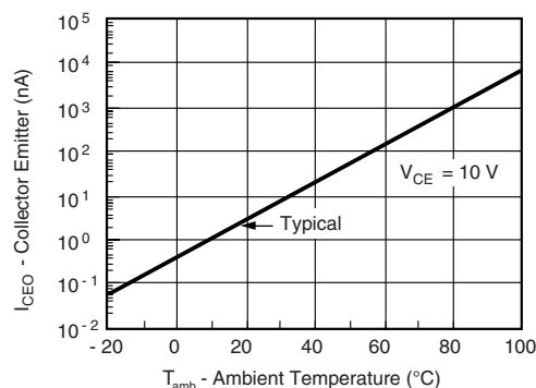
Fig. 9 - Collector Emitter Leakage vs. Temperature
